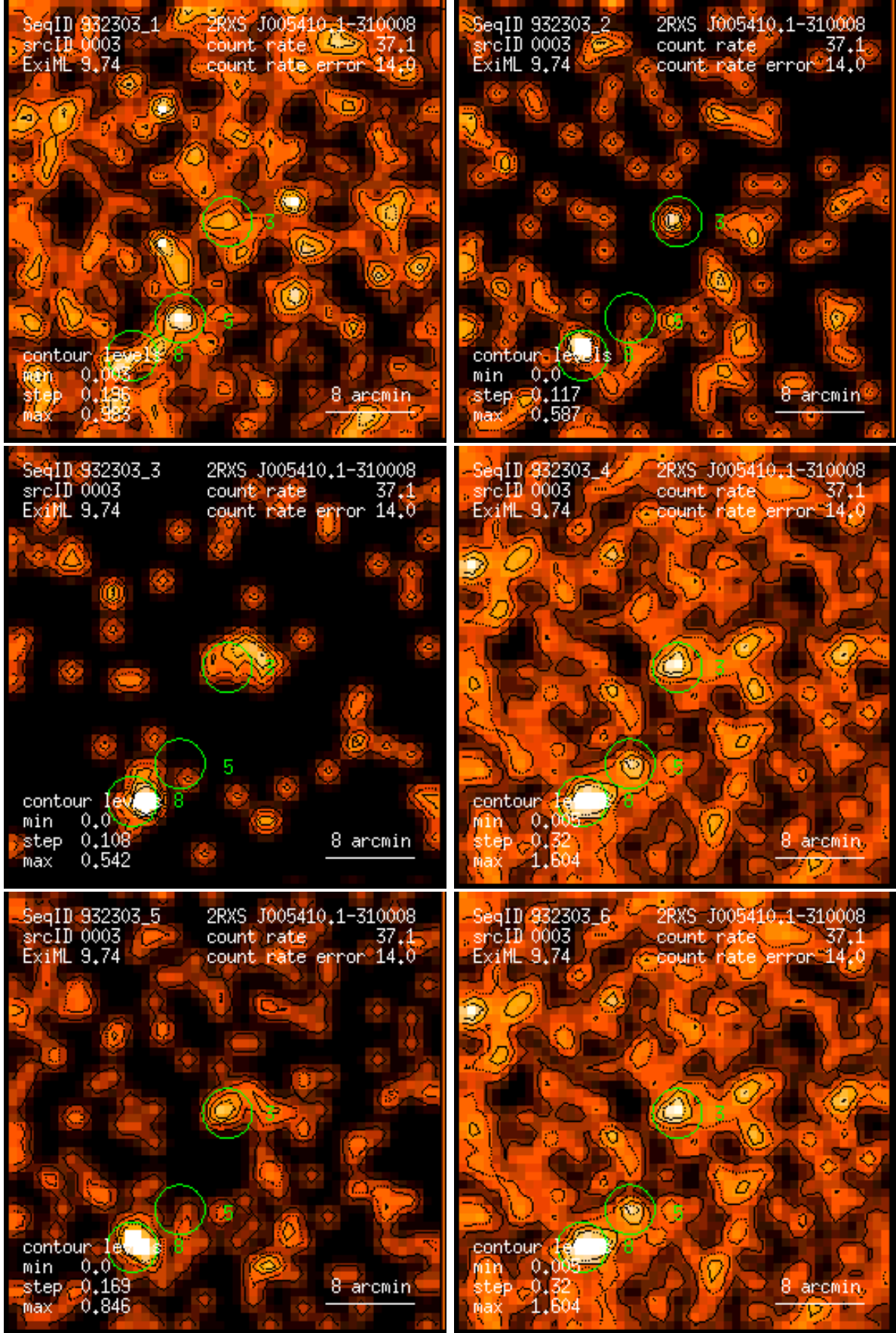
Figure 3: RASS 932303: detection 0003: band rate images, Gaussian filter: (1) PSPC channels 11 – 41, (2) 52 – 90, (3) 91 – 201, (4) 11 – 235, (5) 52 – 201, (6) 11 – 201. Broad band rates in counts/ks. Band rate contour levels in counts/ks/arcmin 2 .
