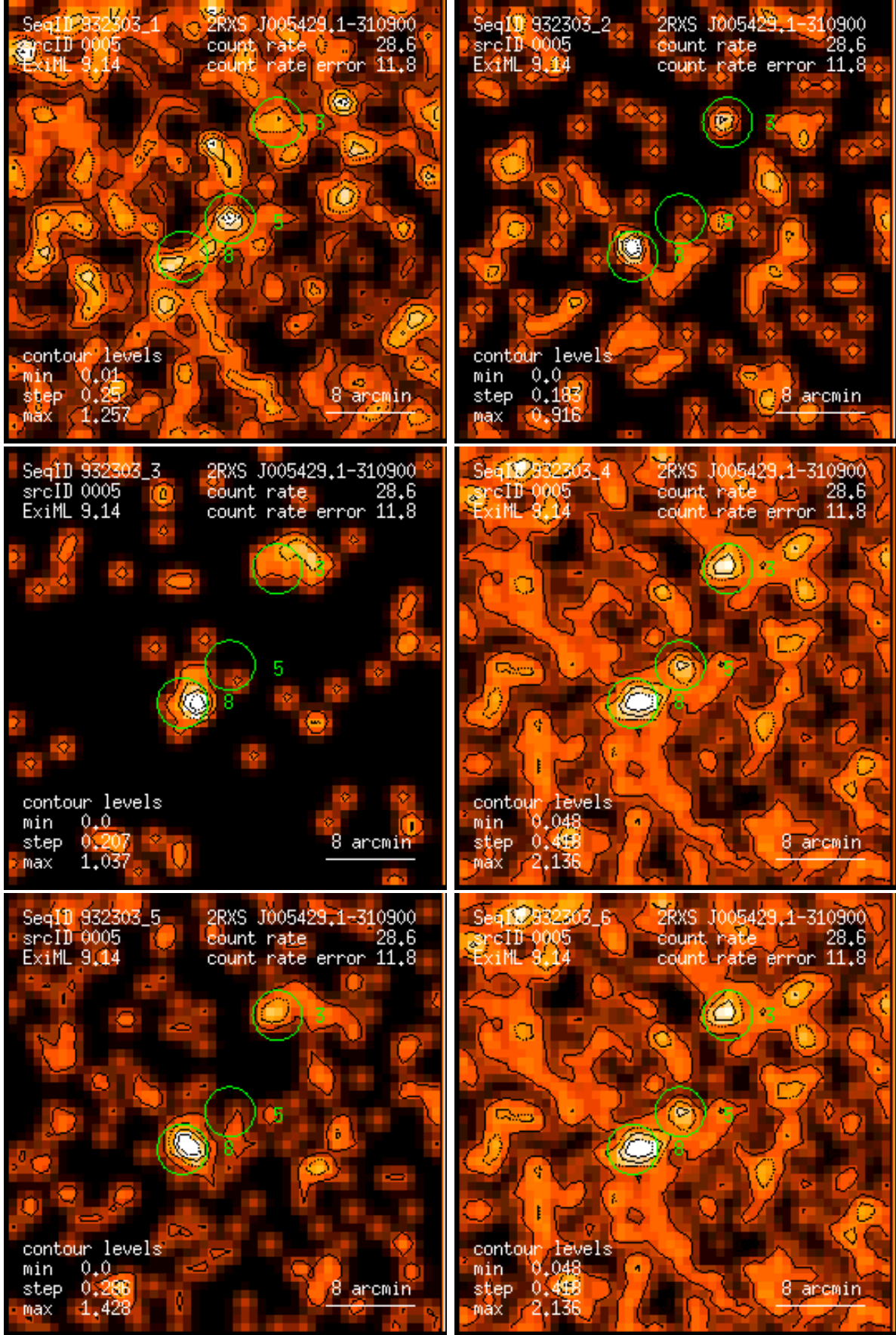
Figure 5: RASS 932303: detection 0005: band rate images, Gaussian filter: (1) PSPC channels 11 – 41, (2) 52 – 90, (3) 91 – 201, (4) 11 – 235, (5) 52 – 201, (6) 11 – 201. Broad band rates in counts/ks. Band rate contour levels in counts/ks/arcmin 2 .
