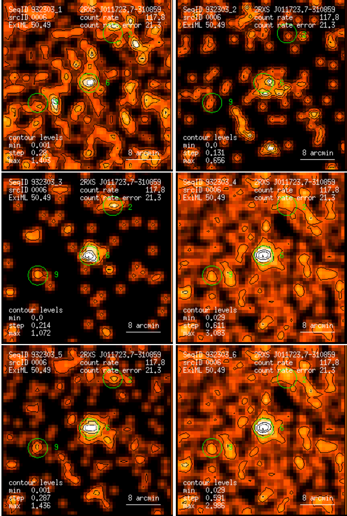
Figure 6: RASS 932303: detection 0006: band rate images, Gaussian filter: (1) PSPC channels 11 – 41, (2) 52 – 90, (3) 91 – 201, (4) 11 – 235, (5) 52 – 201, (6) 11 – 201. Broad band rates in counts/ks. Band rate contour levels in counts/ks/arcmin 2 .
