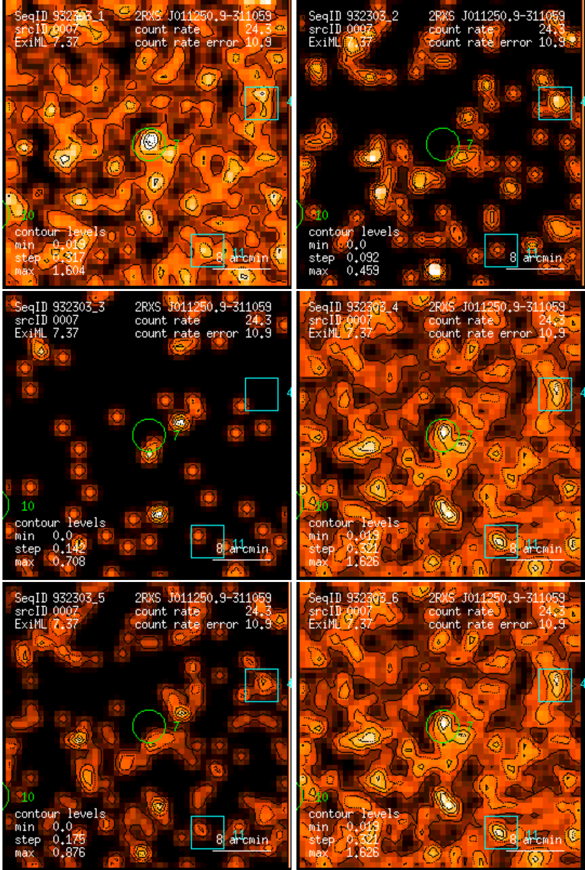
Figure 7: RASS 932303: detection 0007: band rate images, Gaussian filter: (1) PSPC channels 11 – 41, (2) 52 – 90, (3) 91 – 201, (4) 11 – 235, (5) 52 – 201, (6) 11 – 201. Broad band rates in counts/ks. Band rate contour levels in counts/ks/arcmin 2 .
