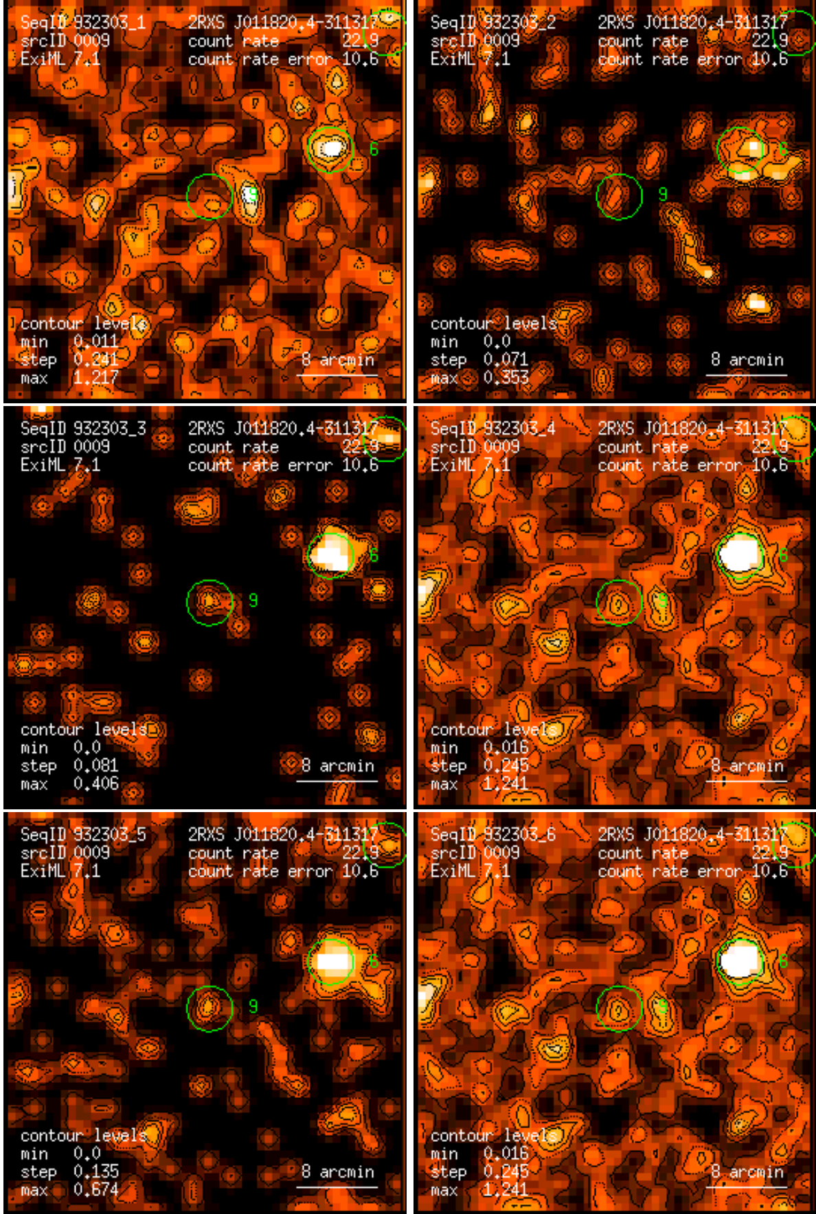
Figure 9: RASS 932303: detection 0009: band rate images, Gaussian filter: (1) PSPC channels 11 – 41, (2) 52 – 90, (3) 91 – 201, (4) 11 – 235, (5) 52 – 201, (6) 11 – 201. Broad band rates in counts/ks. Band rate contour levels in counts/ks/arcmin 2 .
