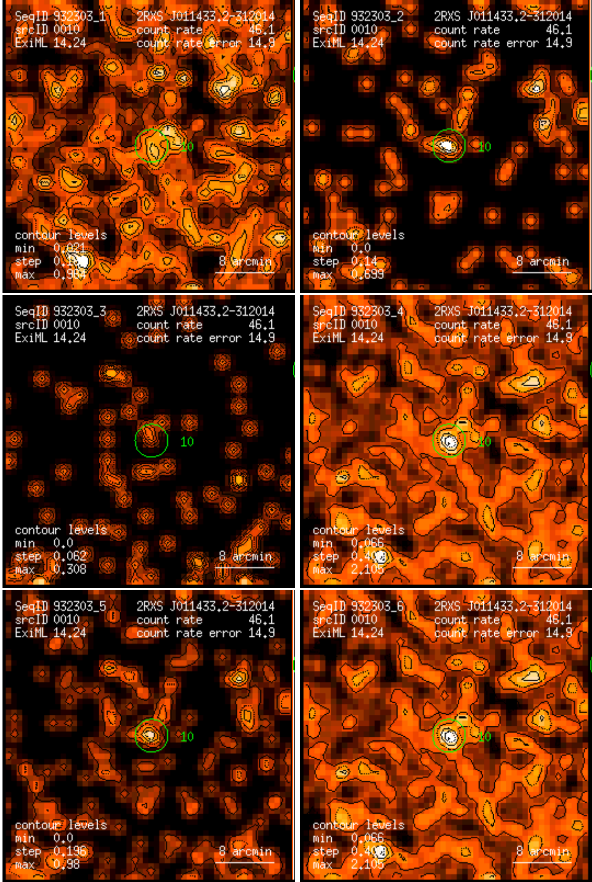
Figure 10: RASS 932303: detection 0010: band rate images, Gaussian filter: (1) PSPC channels 11 – 41, (2) 52 – 90, (3) 91 – 201, (4) 11 – 235, (5) 52 – 201, (6) 11 – 201. Broad band rates in counts/ks. Band rate contour levels in counts/ks/arcmin 2 .
