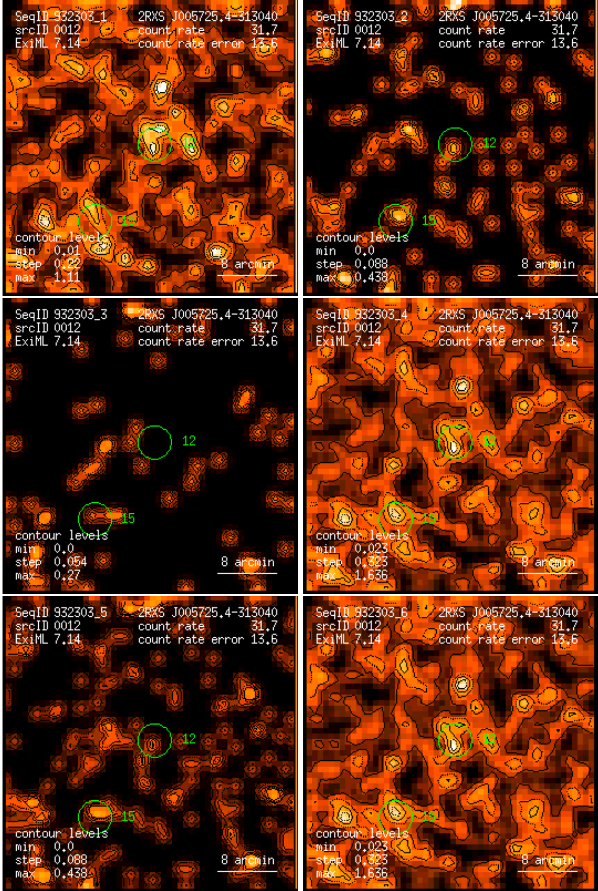
Figure 12: RASS 932303: detection 0012: band rate images, Gaussian filter: (1) PSPC channels 11 – 41, (2) 52 – 90, (3) 91 – 201, (4) 11 – 235, (5) 52 – 201, (6) 11 – 201. Broad band rates in counts/ks. Band rate contour levels in counts/ks/arcmin 2 .
