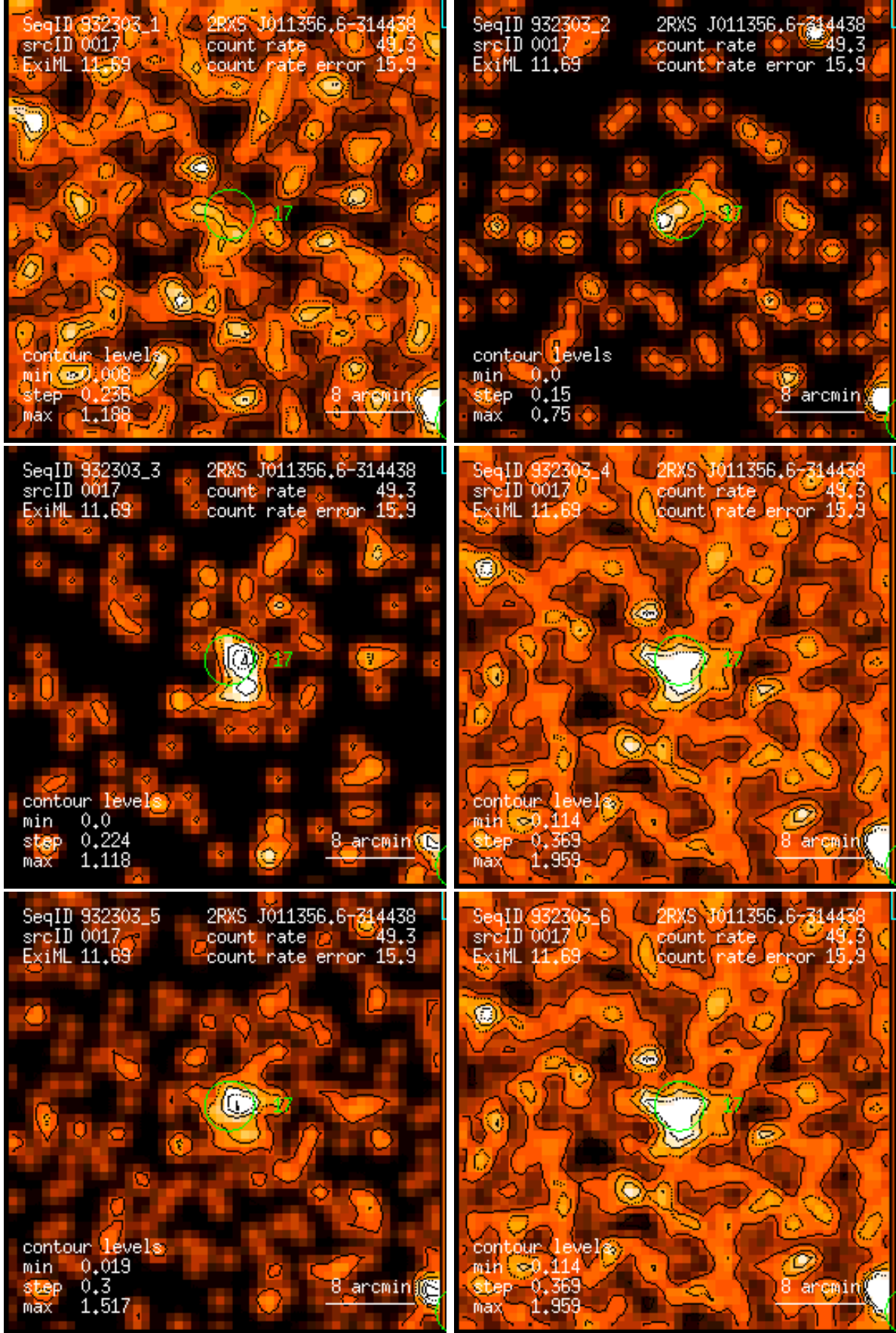
Figure 17: RASS 932303: detection 0017: band rate images, Gaussian filter: (1) PSPC channels 11 – 41, (2) 52 – 90, (3) 91 – 201, (4) 11 – 235, (5) 52 – 201, (6) 11 – 201. Broad band rates in counts/ks. Band rate contour levels in counts/ks/arcmin 2 .
