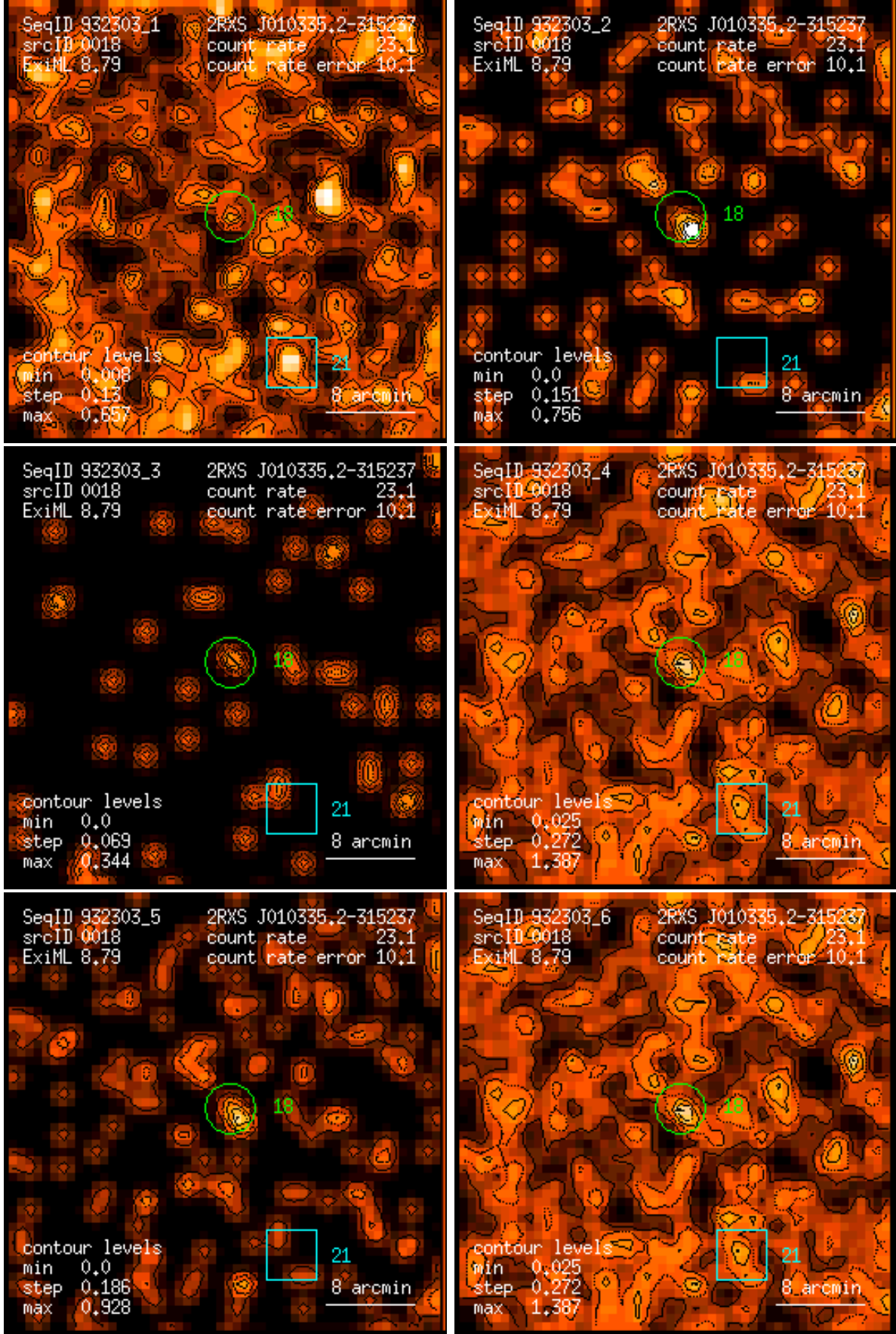
Figure 18: RASS 932303: detection 0018: band rate images, Gaussian filter: (1) PSPC channels 11 – 41, (2) 52 – 90, (3) 91 – 201, (4) 11 – 235, (5) 52 – 201, (6) 11 – 201. Broad band rates in counts/ks. Band rate contour levels in counts/ks/arcmin 2 .
