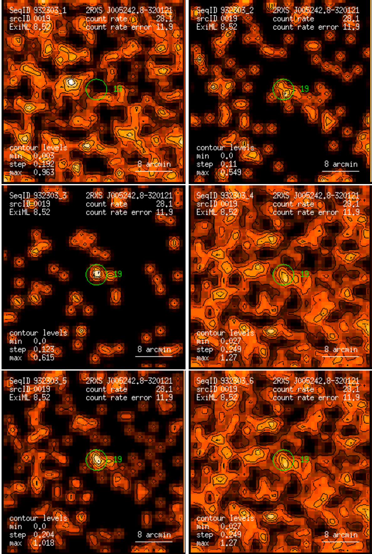
Figure 19: RASS 932303: detection 0019: band rate images, Gaussian filter: (1) PSPC channels 11 – 41, (2) 52 – 90, (3) 91 – 201, (4) 11 – 235, (5) 52 – 201, (6) 11 – 201. Broad band rates in counts/ks. Band rate contour levels in counts/ks/arcmin 2 .
