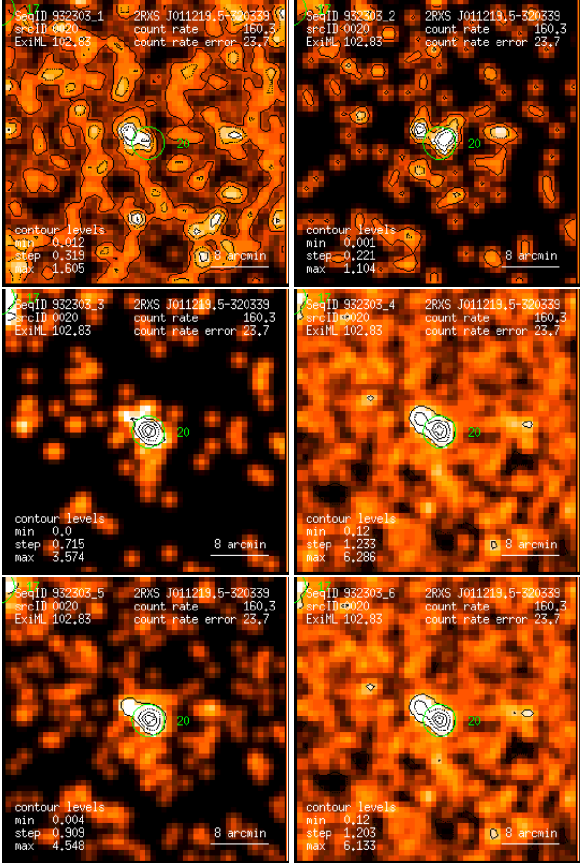
Figure 20: RASS 932303: detection 0020: band rate images, Gaussian filter: (1) PSPC channels 11 – 41, (2) 52 – 90, (3) 91 – 201, (4) 11 – 235, (5) 52 – 201, (6) 11 – 201. Broad band rates in counts/ks. Band rate contour levels in counts/ks/arcmin 2 .
