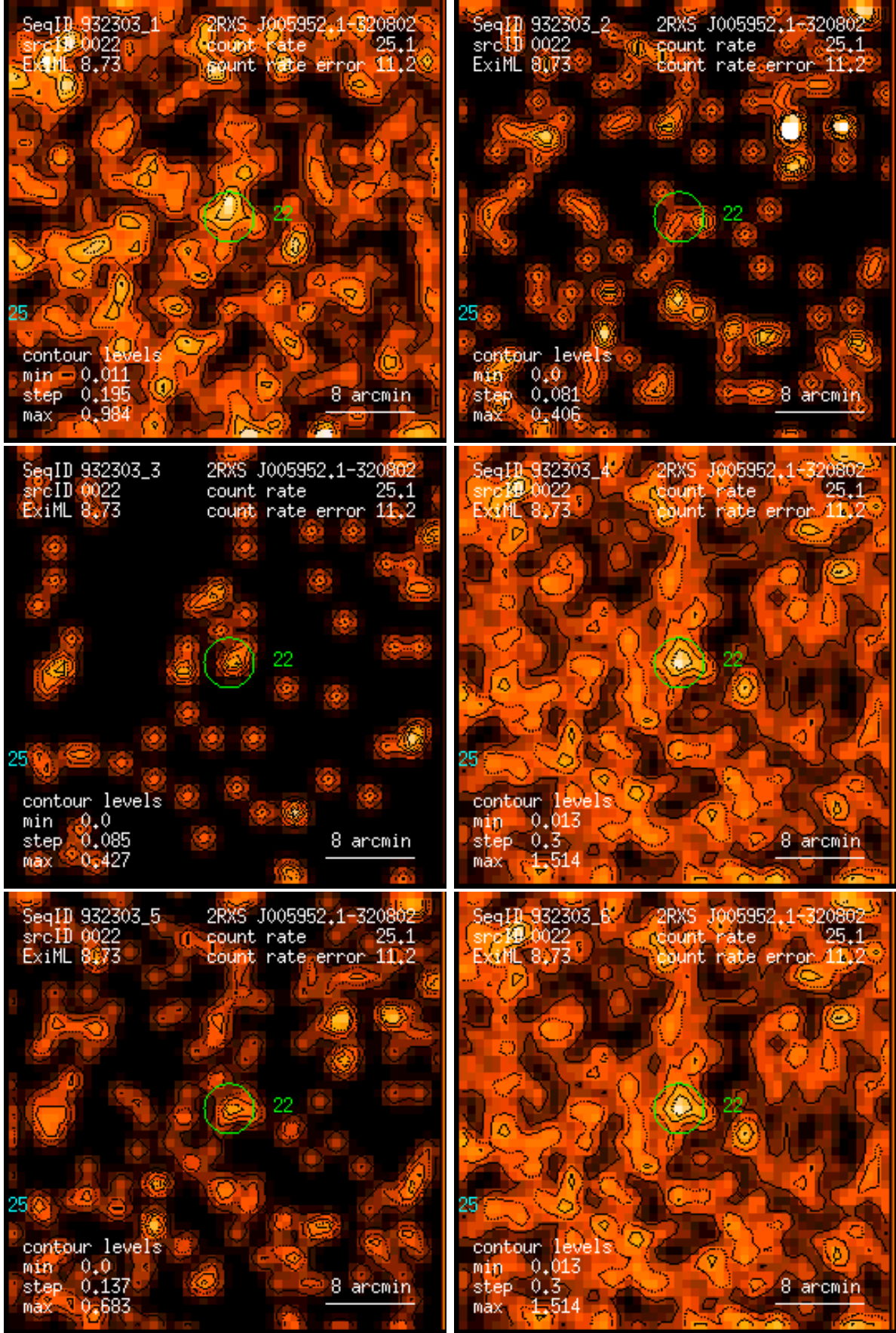
Figure 22: RASS 932303: detection 0022: band rate images, Gaussian filter: (1) PSPC channels 11 – 41, (2) 52 – 90, (3) 91 – 201, (4) 11 – 235, (5) 52 – 201, (6) 11 – 201. Broad band rates in counts/ks. Band rate contour levels in counts/ks/arcmin 2 .
