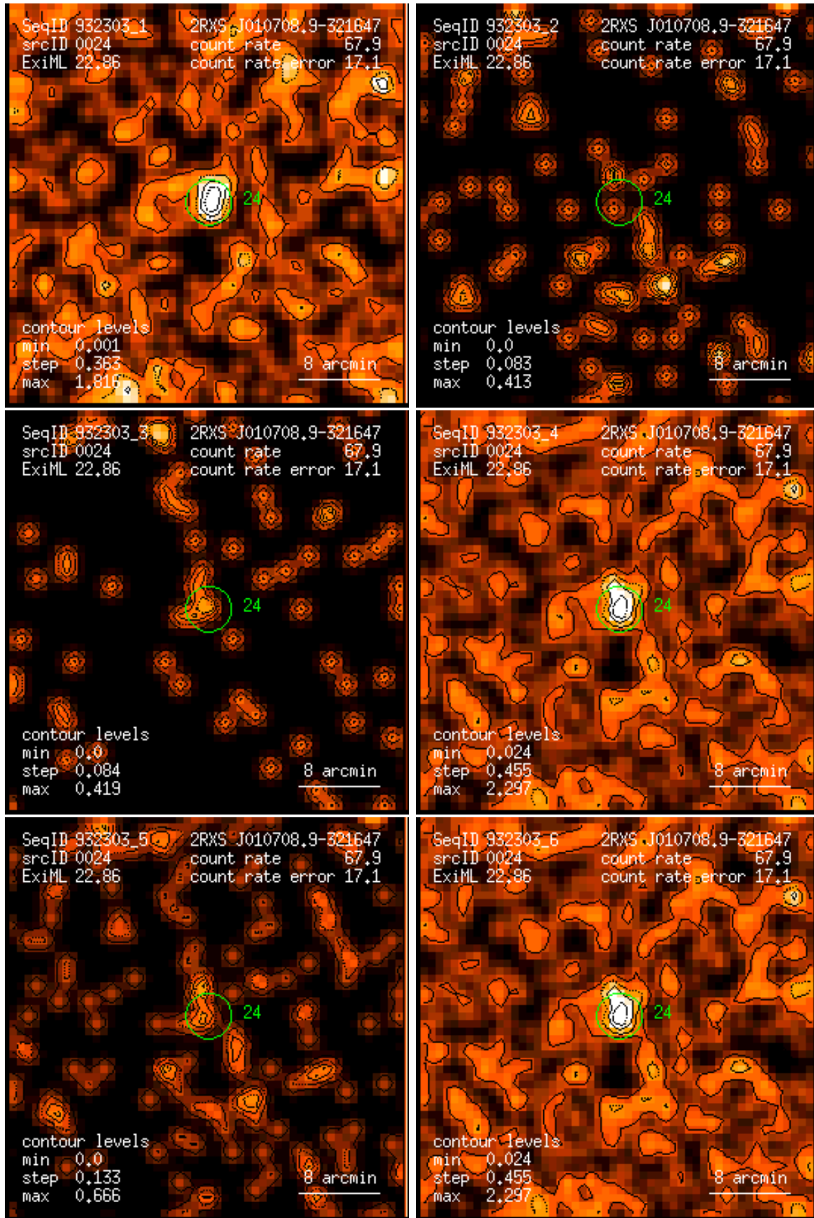
Figure 24: RASS 932303: detection 0024: band rate images, Gaussian filter: (1) PSPC channels 11 – 41, (2) 52 – 90, (3) 91 – 201, (4) 11 – 235, (5) 52 – 201, (6) 11 – 201. Broad band rates in counts/ks. Band rate contour levels in counts/ks/arcmin 2 .
