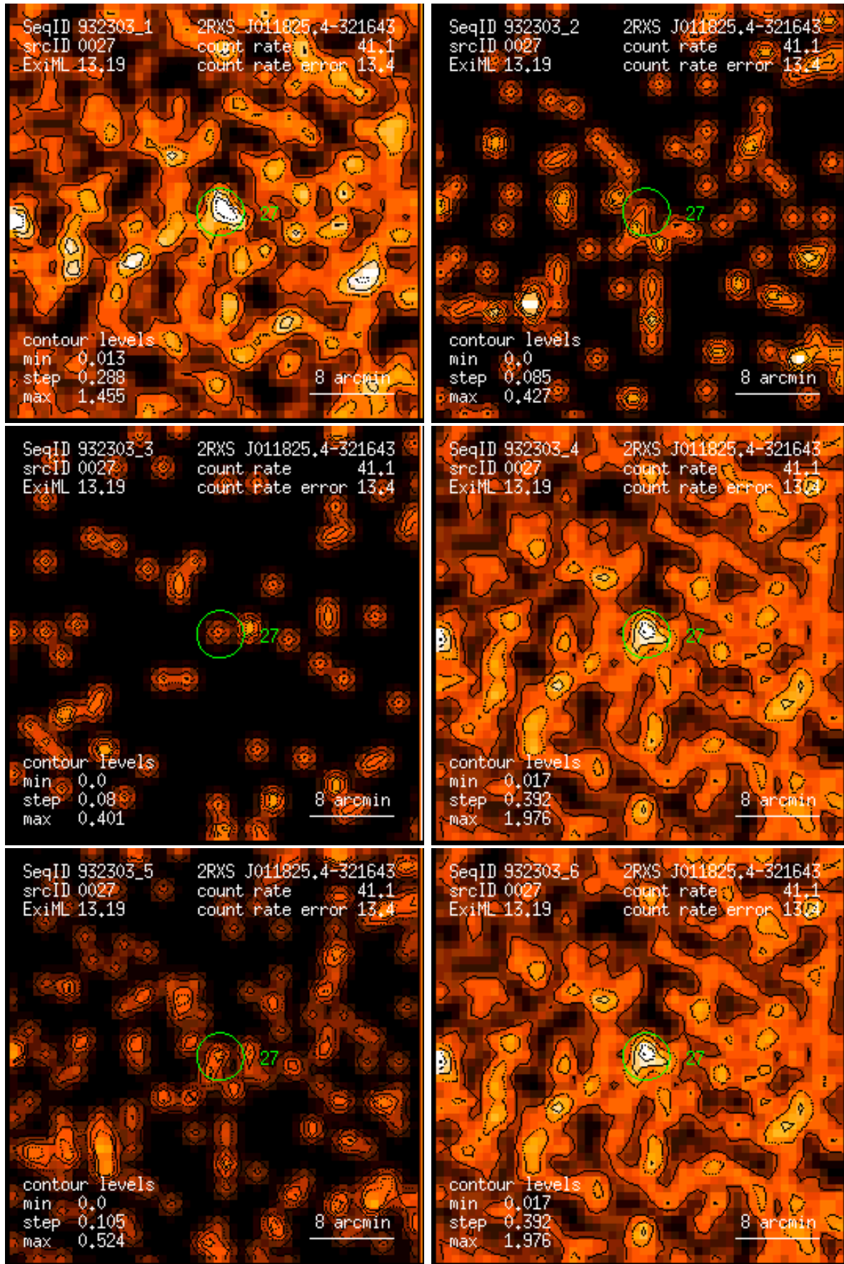
Figure 27: RASS 932303: detection 0027: band rate images, Gaussian filter: (1) PSPC channels 11 – 41, (2) 52 – 90, (3) 91 – 201, (4) 11 – 235, (5) 52 – 201, (6) 11 – 201. Broad band rates in counts/ks. Band rate contour levels in counts/ks/arcmin 2 .
