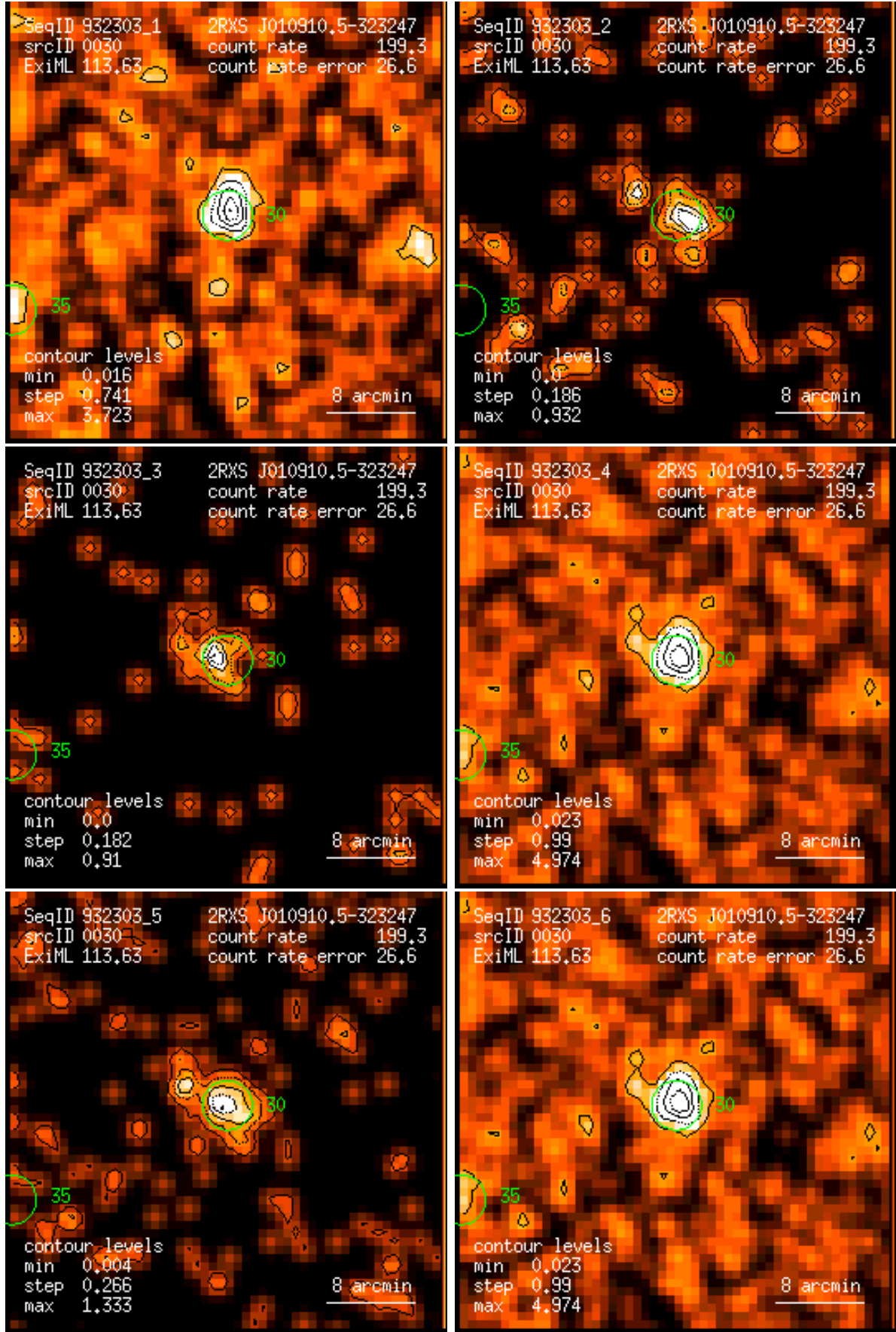
Figure 30: RASS 932303: detection 0030: band rate images, Gaussian filter: (1) PSPC channels 11 – 41, (2) 52 – 90, (3) 91 – 201, (4) 11 – 235, (5) 52 – 201, (6) 11 – 201. Broad band rates in counts/ks. Band rate contour levels in counts/ks/arcmin 2 .
