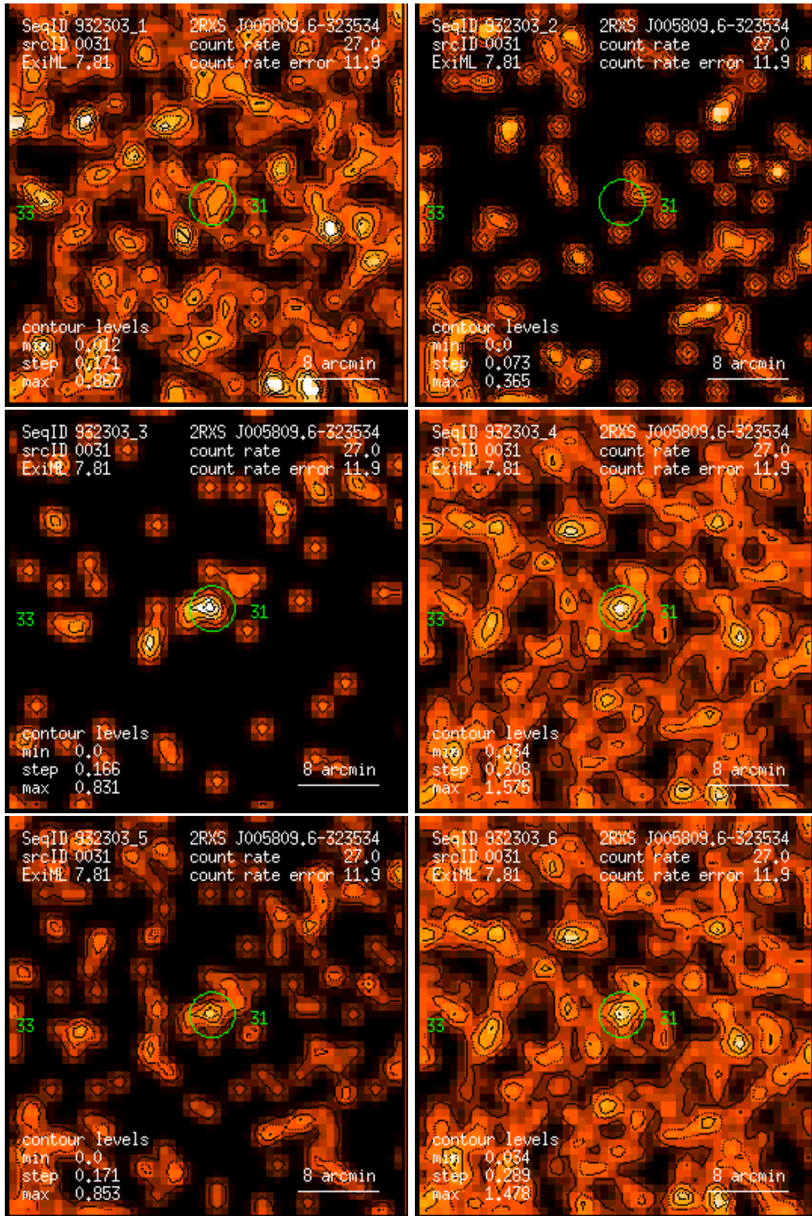
Figure 31: RASS 932303: detection 0031: band rate images, Gaussian filter: (1) PSPC channels 11 – 41, (2) 52 – 90, (3) 91 – 201, (4) 11 – 235, (5) 52 – 201, (6) 11 – 201. Broad band rates in counts/ks. Band rate contour levels in counts/ks/arcmin 2 .
