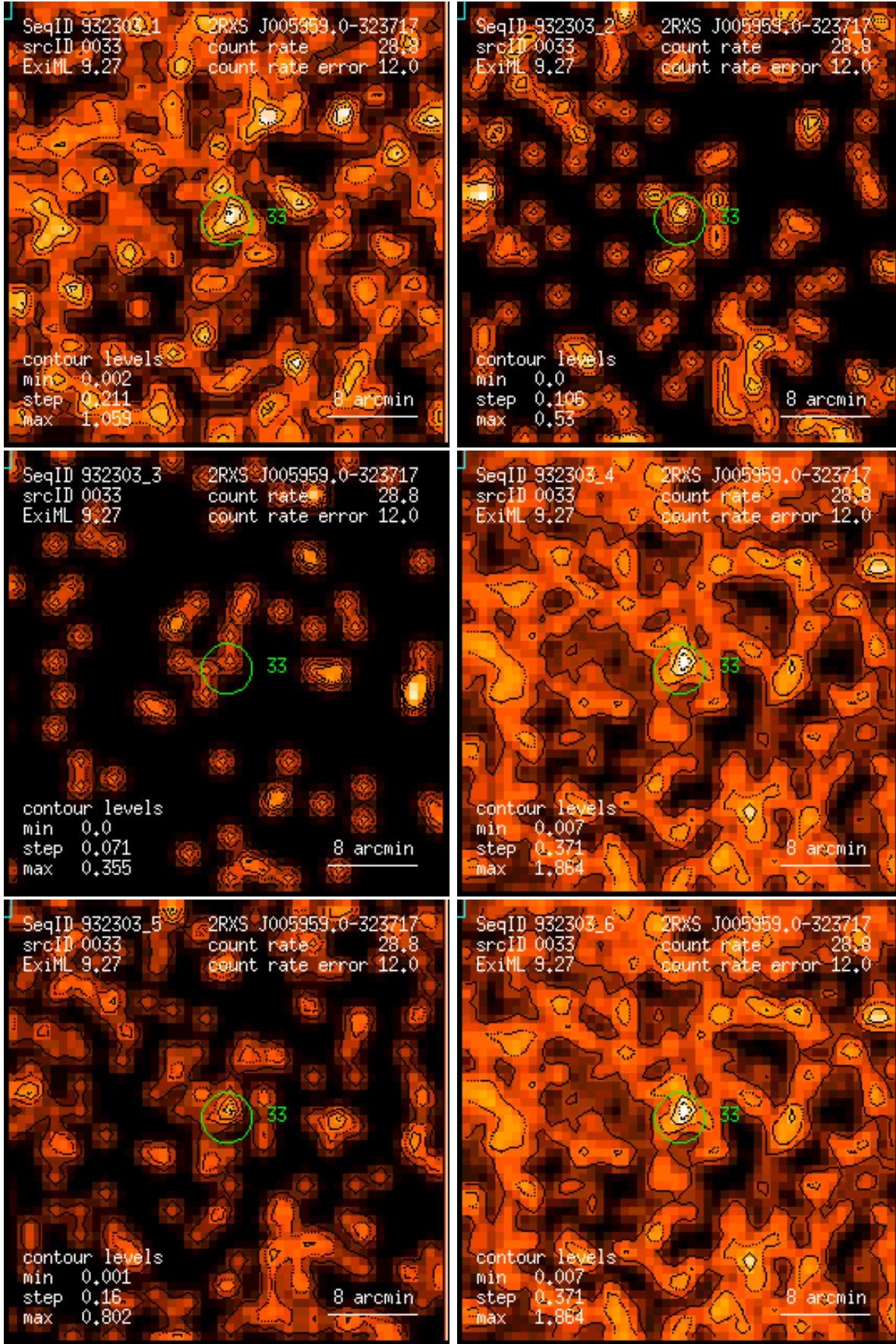
Figure 33: RASS 932303: detection 0033: band rate images, Gaussian filter: (1) PSPC channels 11 – 41, (2) 52 – 90, (3) 91 – 201, (4) 11 – 235, (5) 52 – 201, (6) 11 – 201. Broad band rates in counts/ks. Band rate contour levels in counts/ks/arcmin 2 .
