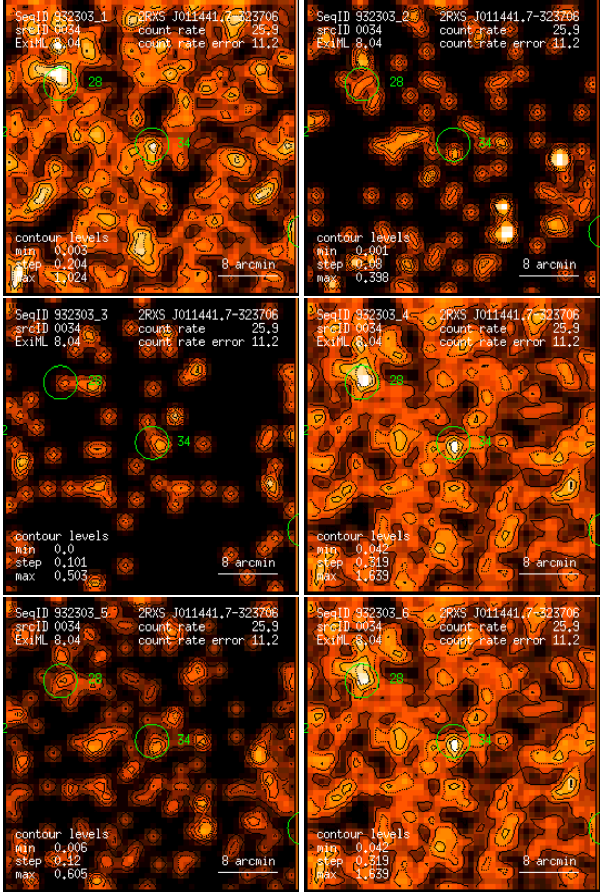
Figure 34: RASS 932303: detection 0034: band rate images, Gaussian filter: (1) PSPC channels 11 – 41, (2) 52 – 90, (3) 91 – 201, (4) 11 – 235, (5) 52 – 201, (6) 11 – 201. Broad band rates in counts/ks. Band rate contour levels in counts/ks/arcmin 2 .
