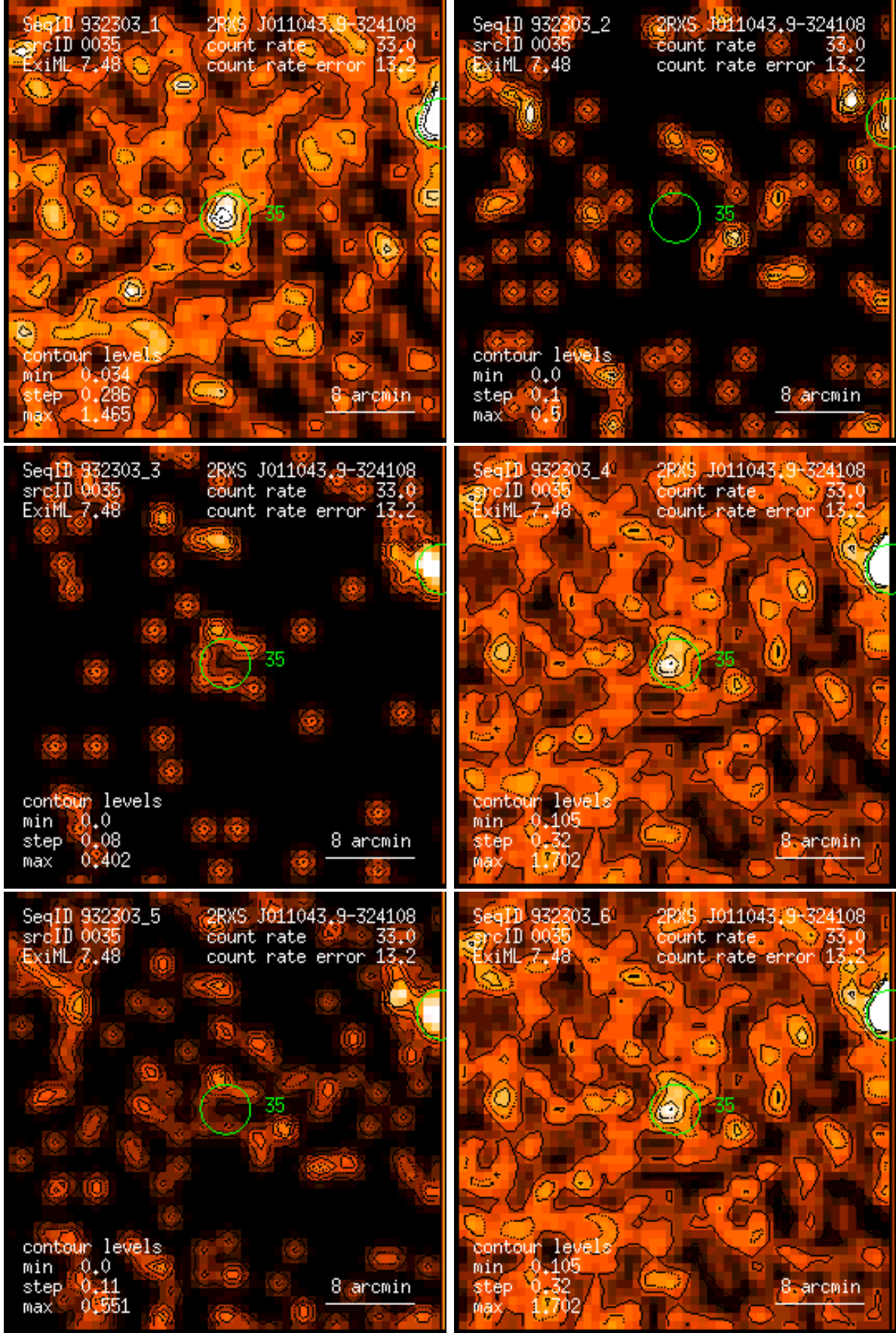
Figure 35: RASS 932303: detection 0035: band rate images, Gaussian filter: (1) PSPC channels 11 – 41, (2) 52 – 90, (3) 91 – 201, (4) 11 – 235, (5) 52 – 201, (6) 11 – 201. Broad band rates in counts/ks. Band rate contour levels in counts/ks/arcmin 2 .
