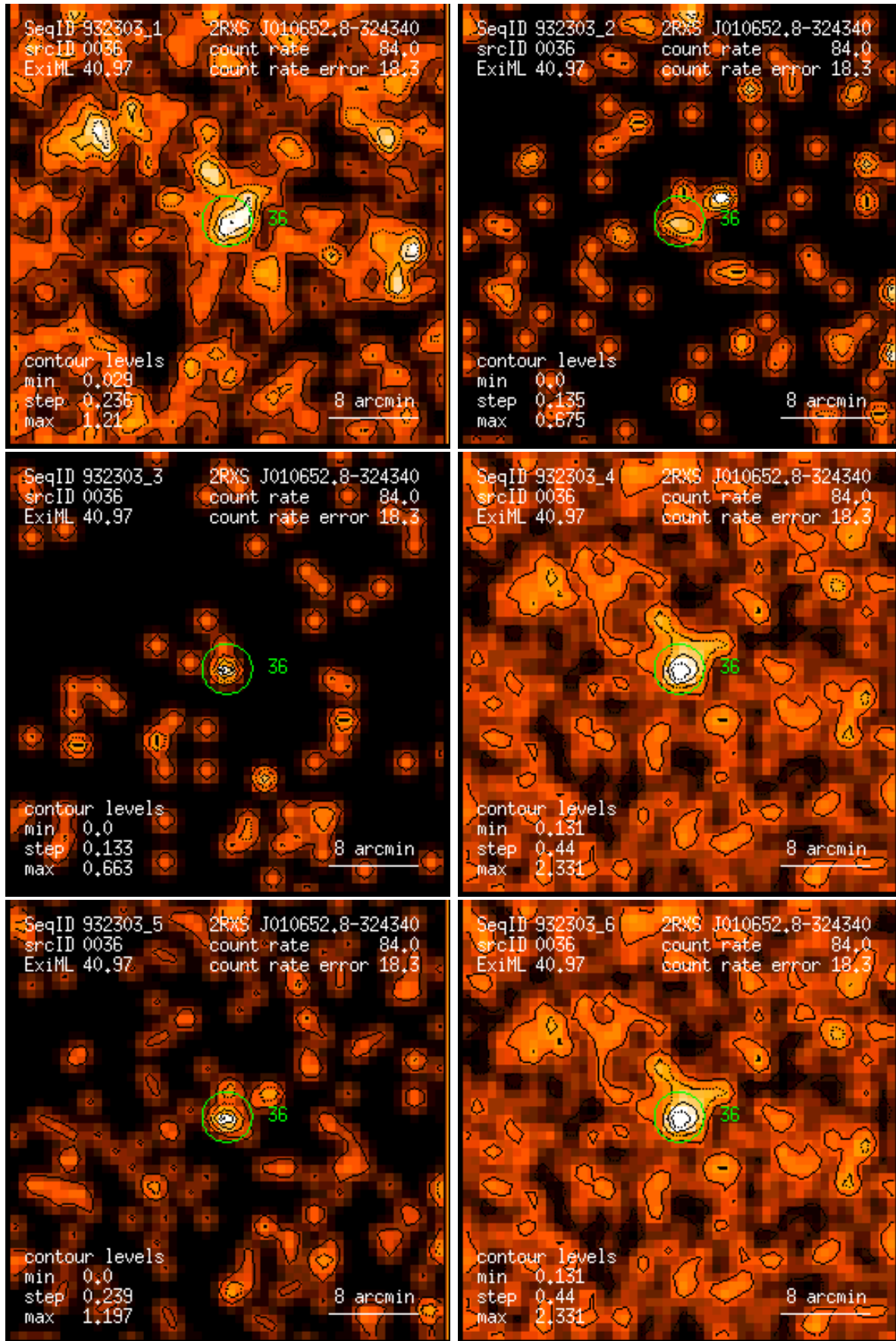
Figure 36: RASS 932303: detection 0036: band rate images, Gaussian filter: (1) PSPC channels 11 – 41, (2) 52 – 90, (3) 91 – 201, (4) 11 – 235, (5) 52 – 201, (6) 11 – 201. Broad band rates in counts/ks. Band rate contour levels in counts/ks/arcmin 2 .
