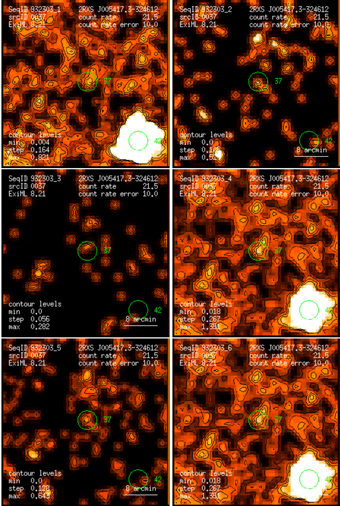
Figure 37: RASS 932303: detection 0037: band rate images, Gaussian filter: (1) PSPC channels 11 – 41, (2) 52 – 90, (3) 91 – 201, (4) 11 – 235, (5) 52 – 201, (6) 11 – 201. Broad band rates in counts/ks. Band rate contour levels in counts/ks/arcmin 2 .
