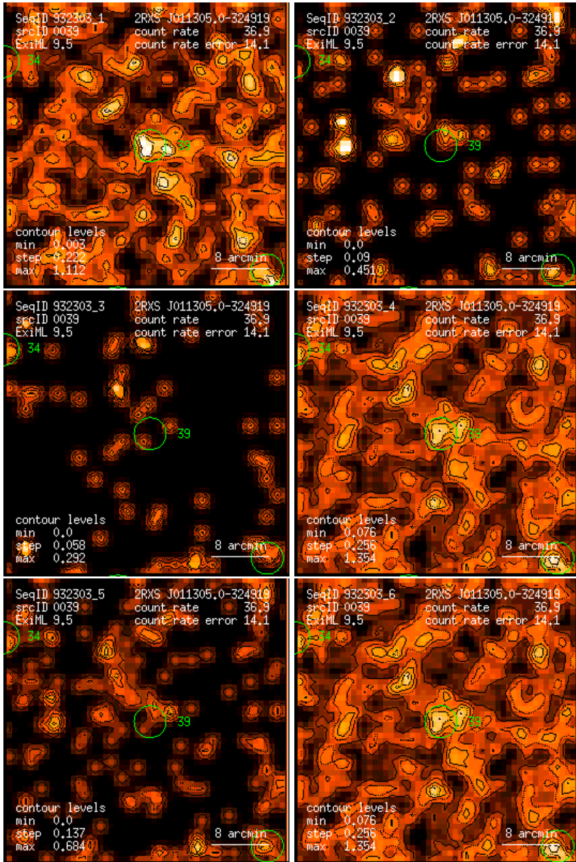
Figure 39: RASS 932303: detection 0039: band rate images, Gaussian filter: (1) PSPC channels 11 – 41, (2) 52 – 90, (3) 91 – 201, (4) 11 – 235, (5) 52 – 201, (6) 11 – 201. Broad band rates in counts/ks. Band rate contour levels in counts/ks/arcmin 2 .
