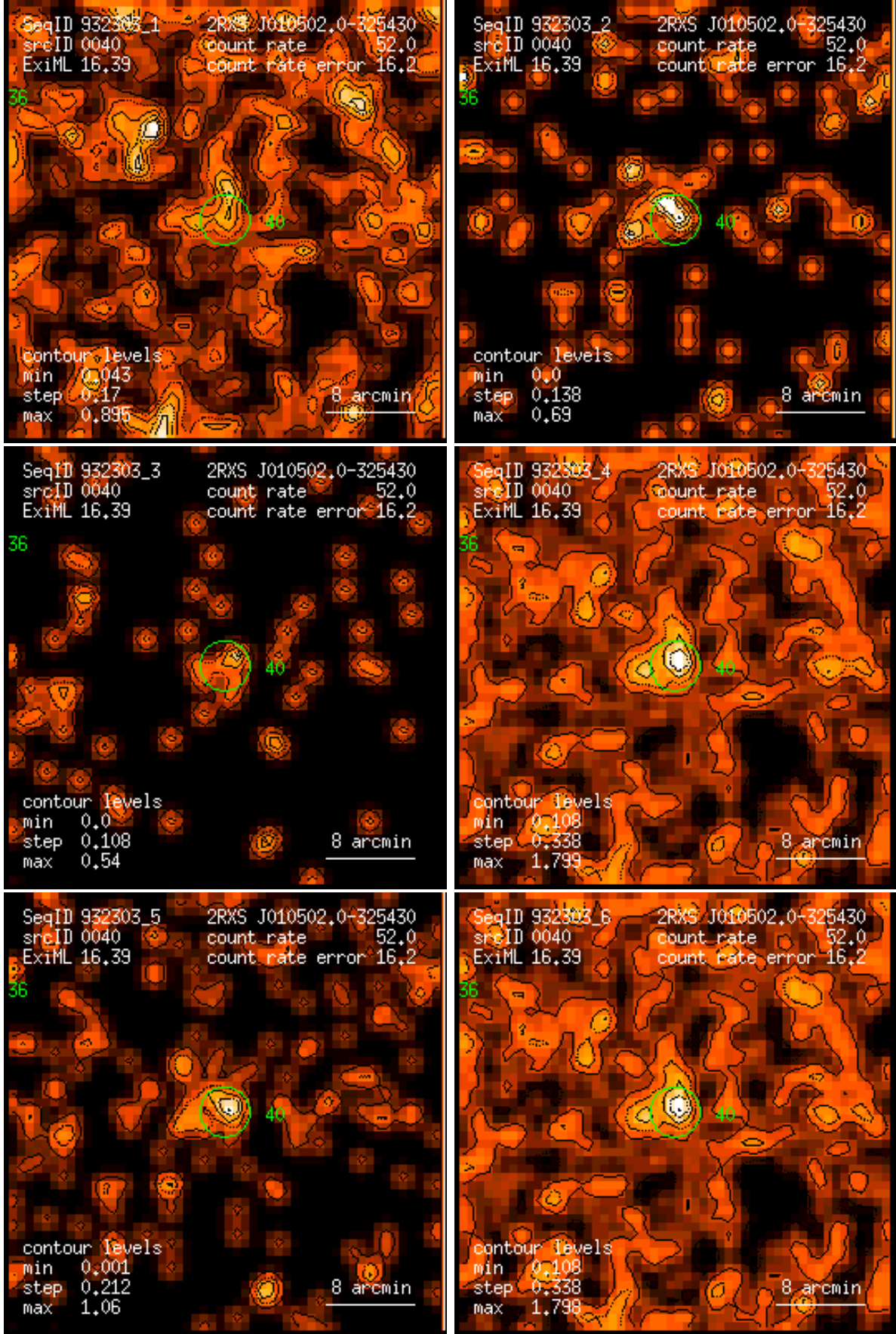
Figure 40: RASS 932303: detection 0040: band rate images, Gaussian filter: (1) PSPC channels 11 – 41, (2) 52 – 90, (3) 91 – 201, (4) 11 – 235, (5) 52 – 201, (6) 11 – 201. Broad band rates in counts/ks. Band rate contour levels in counts/ks/arcmin 2 .
