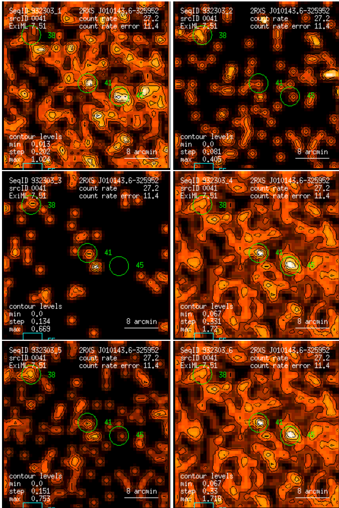
Figure 41: RASS 932303: detection 0041: band rate images, Gaussian filter: (1) PSPC channels 11 – 41, (2) 52 – 90, (3) 91 – 201, (4) 11 – 235, (5) 52 – 201, (6) 11 – 201. Broad band rates in counts/ks. Band rate contour levels in counts/ks/arcmin 2 .
