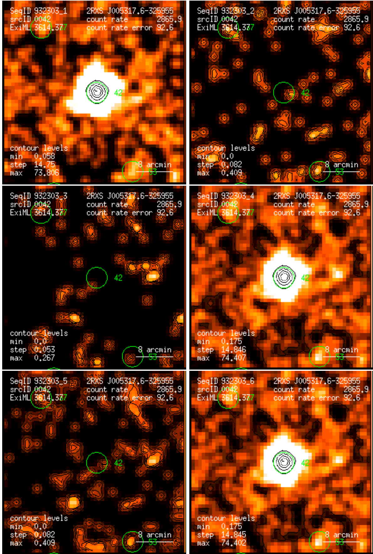
Figure 42: RASS 932303: detection 0042: band rate images, Gaussian filter: (1) PSPC channels 11 – 41, (2) 52 – 90, (3) 91 – 201, (4) 11 – 235, (5) 52 – 201, (6) 11 – 201. Broad band rates in counts/ks. Band rate contour levels in counts/ks/arcmin 2 .
