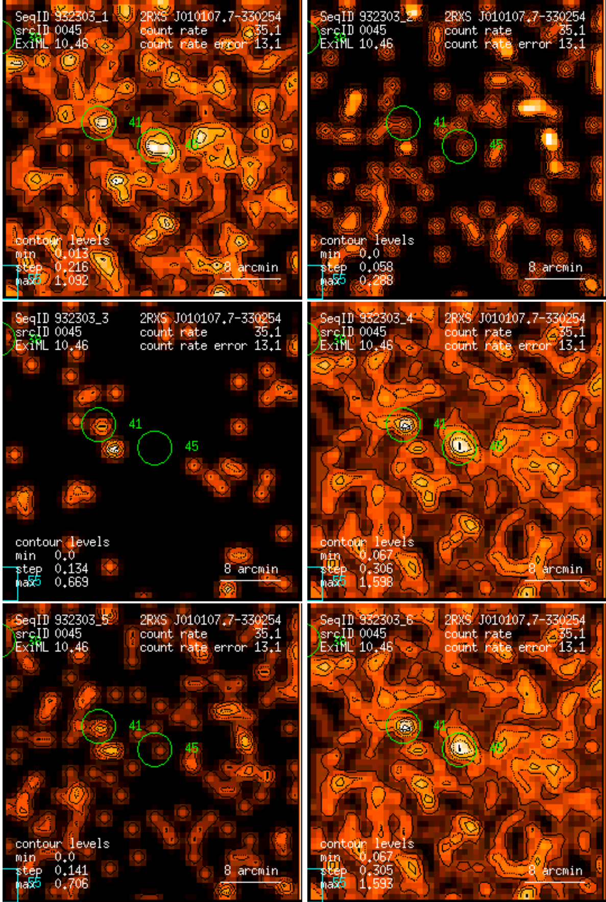
Figure 45: RASS 932303: detection 0045: band rate images, Gaussian filter: (1) PSPC channels 11 – 41, (2) 52 – 90, (3) 91 – 201, (4) 11 – 235, (5) 52 – 201, (6) 11 – 201. Broad band rates in counts/ks. Band rate contour levels in counts/ks/arcmin 2 .
