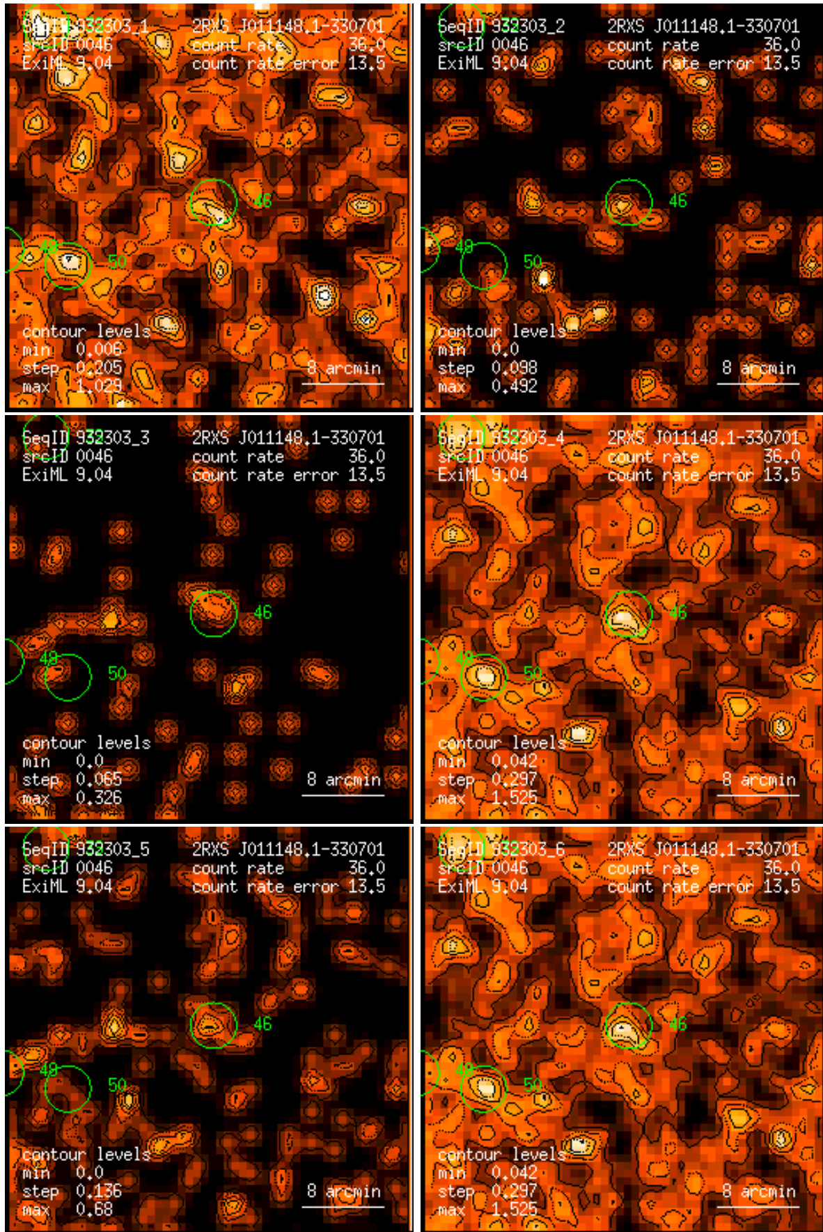
Figure 46: RASS 932303: detection 0046: band rate images, Gaussian filter: (1) PSPC channels 11 – 41, (2) 52 – 90, (3) 91 – 201, (4) 11 – 235, (5) 52 – 201, (6) 11 – 201. Broad band rates in counts/ks. Band rate contour levels in counts/ks/arcmin 2 .
