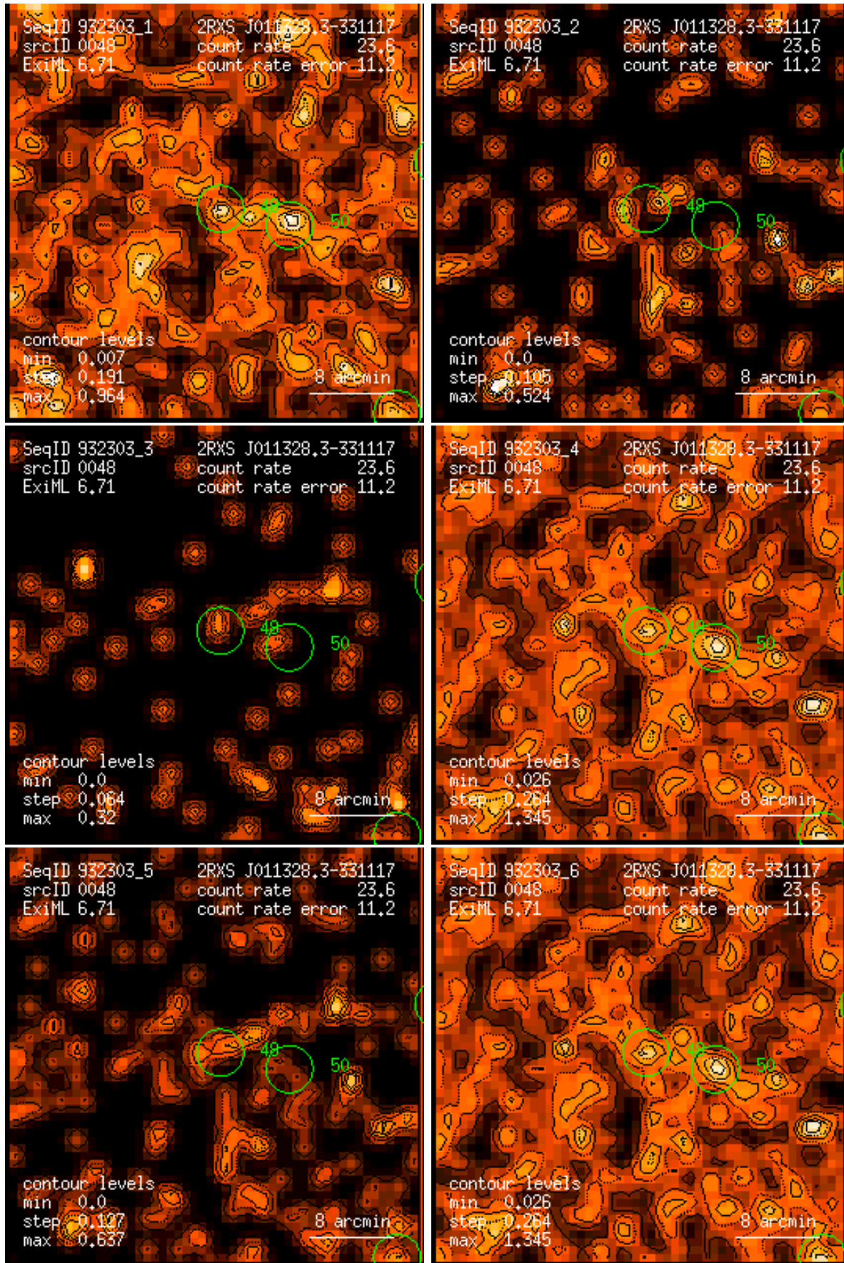
Figure 48: RASS 932303: detection 0048: band rate images, Gaussian filter: (1) PSPC channels 11 – 41, (2) 52 – 90, (3) 91 – 201, (4) 11 – 235, (5) 52 – 201, (6) 11 – 201. Broad band rates in counts/ks. Band rate contour levels in counts/ks/arcmin 2 .
