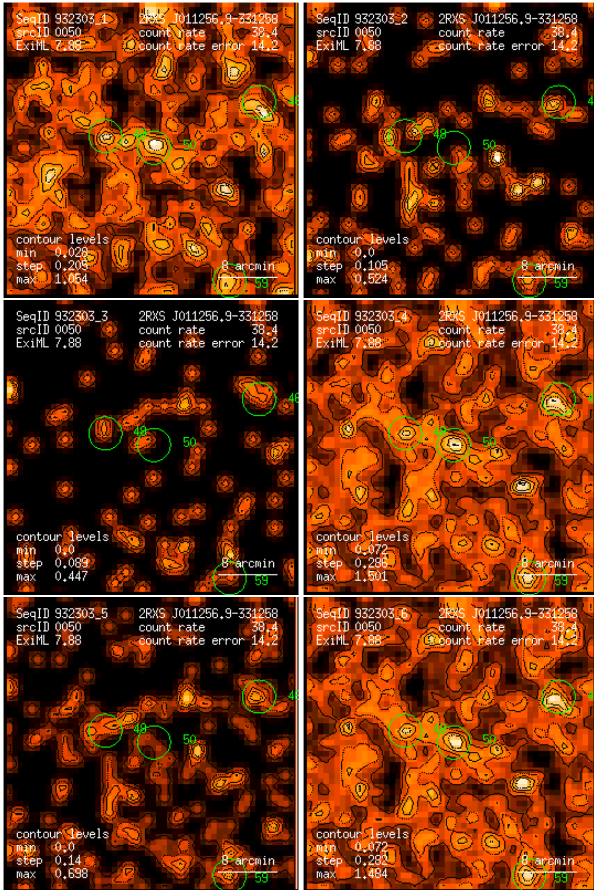
Figure 50: RASS 932303: detection 0050: band rate images, Gaussian filter: (1) PSPC channels 11 – 41, (2) 52 – 90, (3) 91 – 201, (4) 11 – 235, (5) 52 – 201, (6) 11 – 201. Broad band rates in counts/ks. Band rate contour levels in counts/ks/arcmin 2 .
