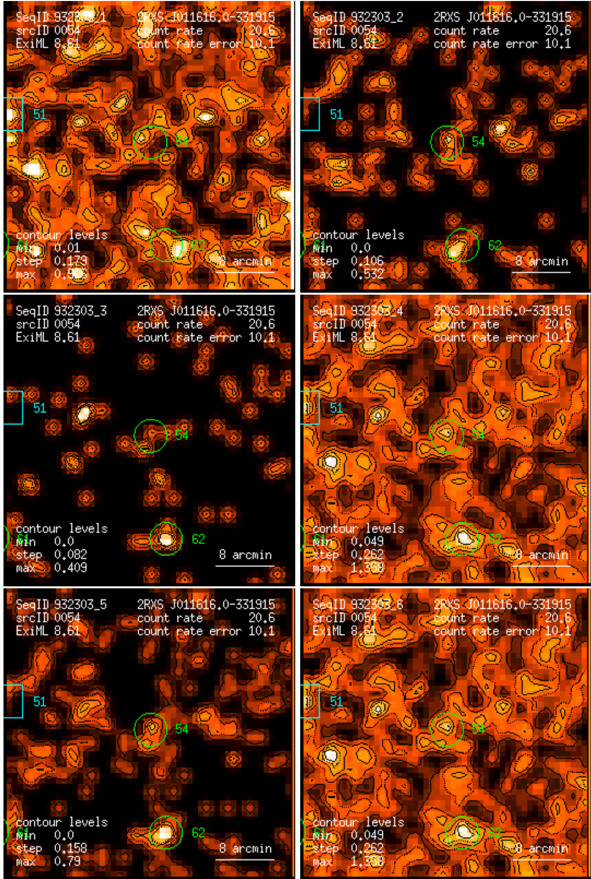
Figure 54: RASS 932303: detection 0054: band rate images, Gaussian filter: (1) PSPC channels 11 – 41, (2) 52 – 90, (3) 91 – 201, (4) 11 – 235, (5) 52 – 201, (6) 11 – 201. Broad band rates in counts/ks. Band rate contour levels in counts/ks/arcmin 2 .
