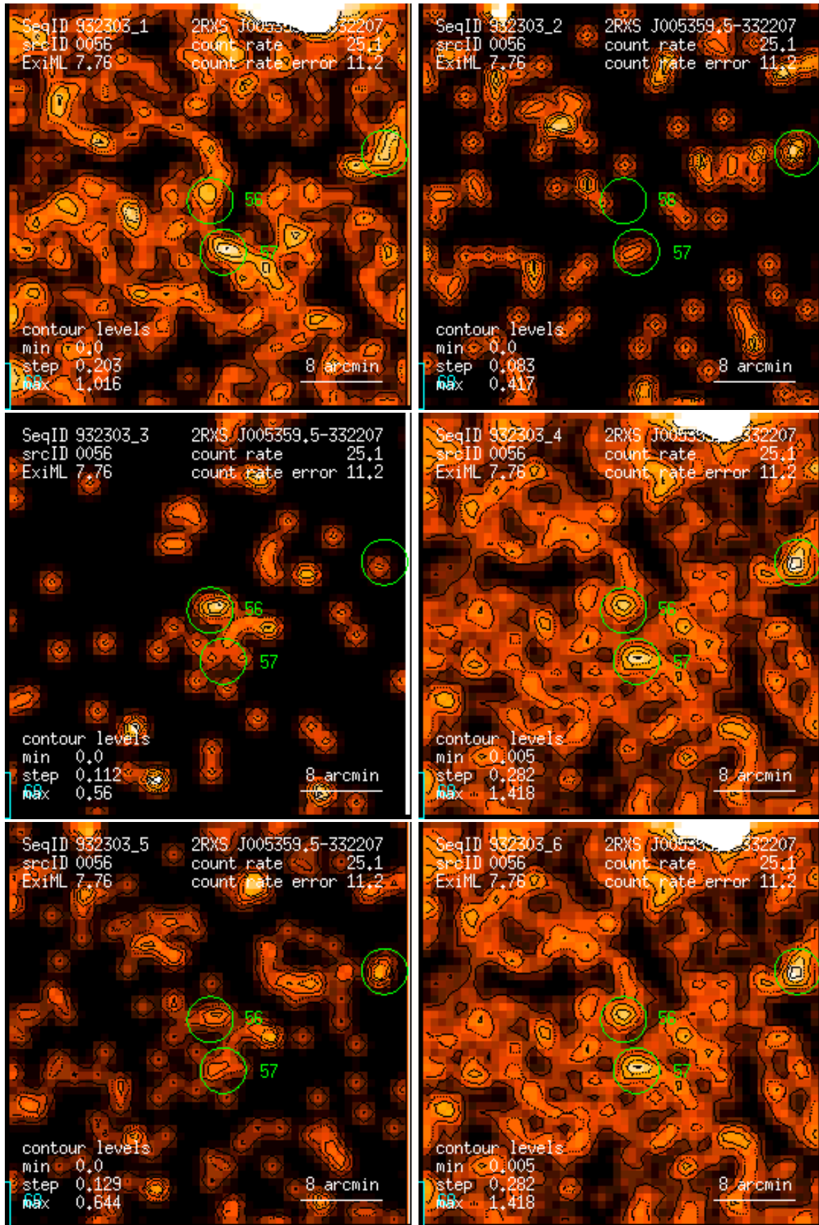
Figure 56: RASS 932303: detection 0056: band rate images, Gaussian filter: (1) PSPC channels 11 – 41, (2) 52 – 90, (3) 91 – 201, (4) 11 – 235, (5) 52 – 201, (6) 11 – 201. Broad band rates in counts/ks. Band rate contour levels in counts/ks/arcmin 2 .
