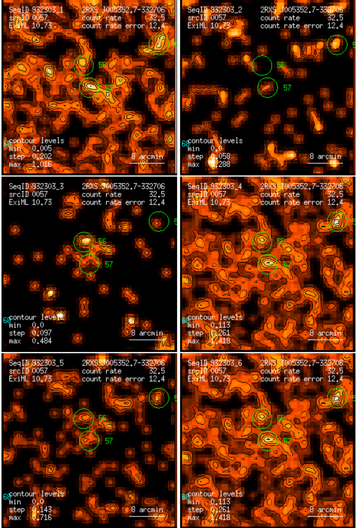
Figure 57: RASS 932303: detection 0057: band rate images, Gaussian filter: (1) PSPC channels 11 – 41, (2) 52 – 90, (3) 91 – 201, (4) 11 – 235, (5) 52 – 201, (6) 11 – 201. Broad band rates in counts/ks. Band rate contour levels in counts/ks/arcmin 2 .
