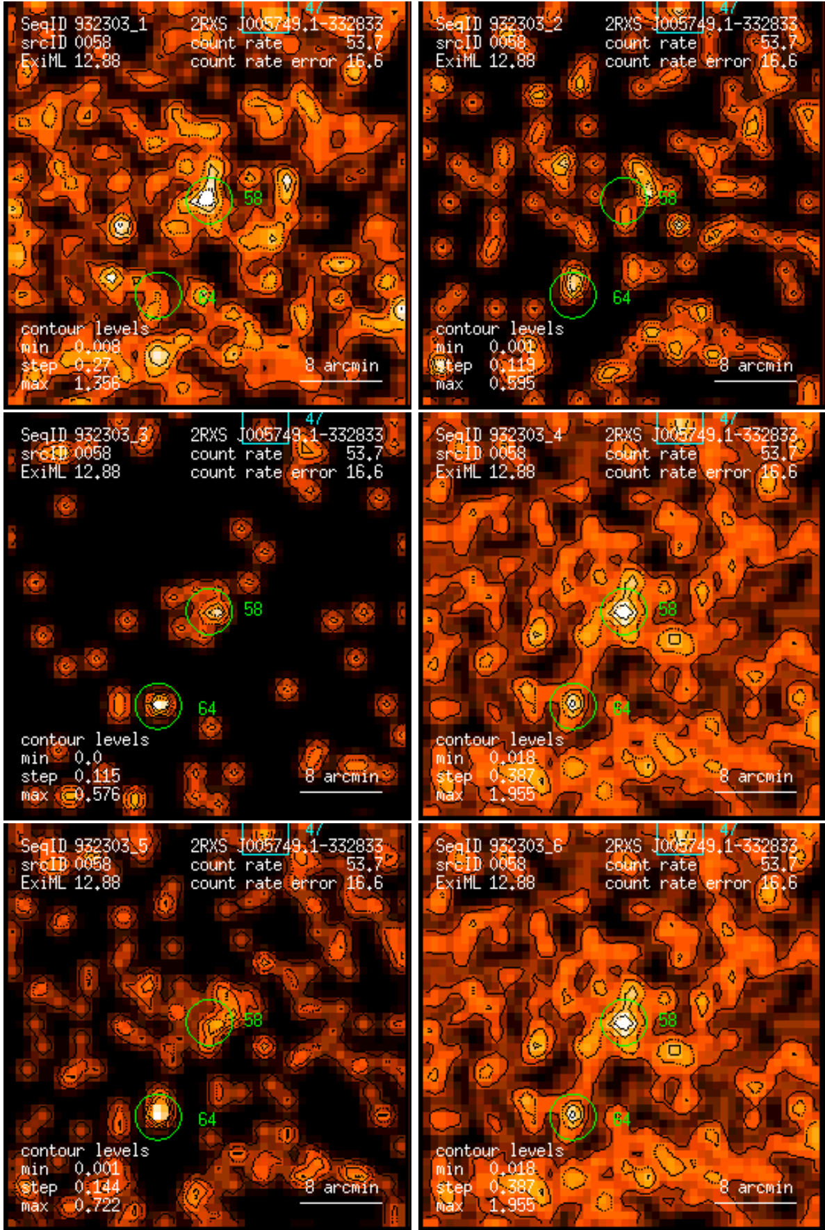
Figure 58: RASS 932303: detection 0058: band rate images, Gaussian filter: (1) PSPC channels 11 – 41, (2) 52 – 90, (3) 91 – 201, (4) 11 – 235, (5) 52 – 201, (6) 11 – 201. Broad band rates in counts/ks. Band rate contour levels in counts/ks/arcmin 2 .
