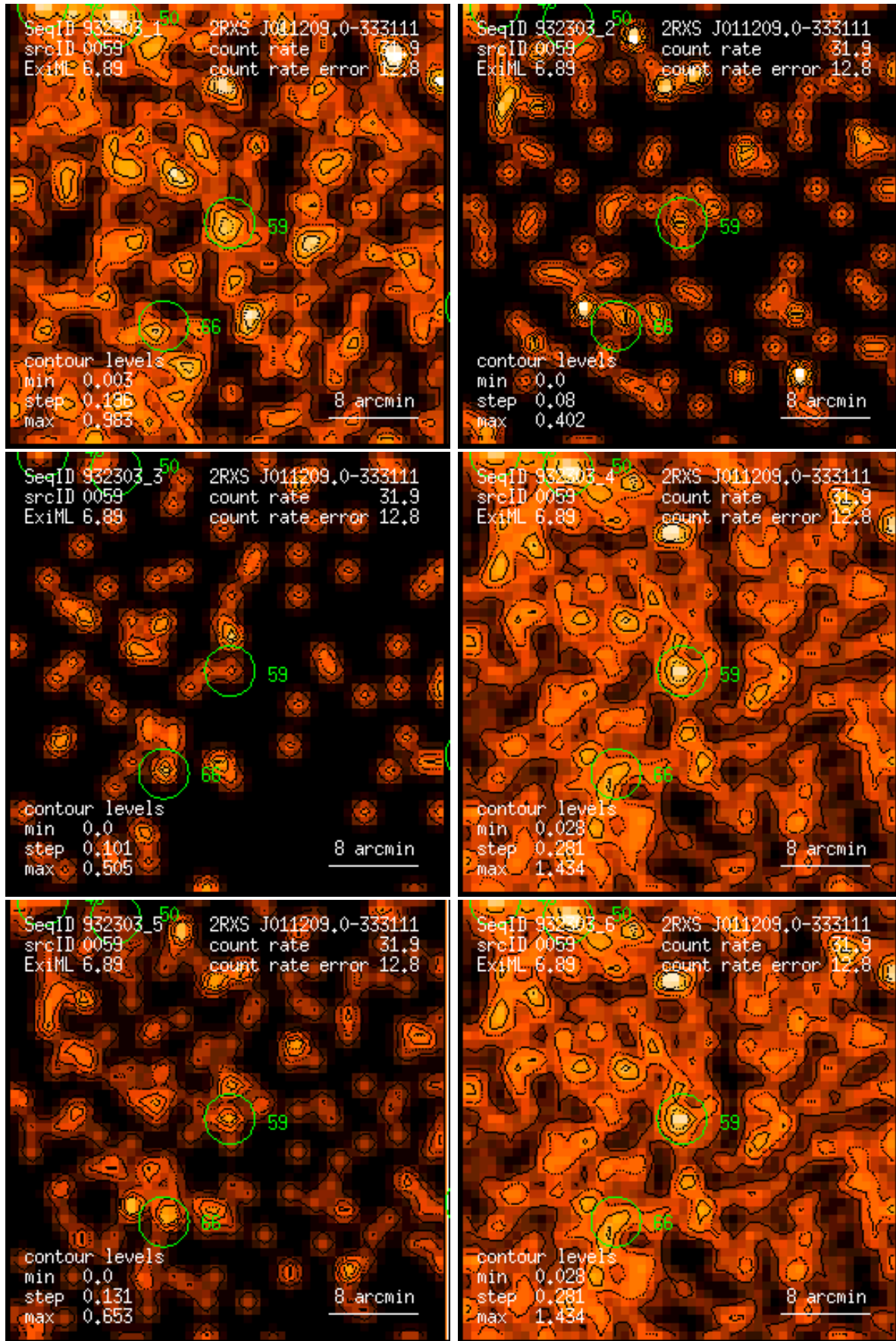
Figure 59: RASS 932303: detection 0059: band rate images, Gaussian filter: (1) PSPC channels 11 – 41, (2) 52 – 90, (3) 91 – 201, (4) 11 – 235, (5) 52 – 201, (6) 11 – 201. Broad band rates in counts/ks. Band rate contour levels in counts/ks/arcmin 2 .
