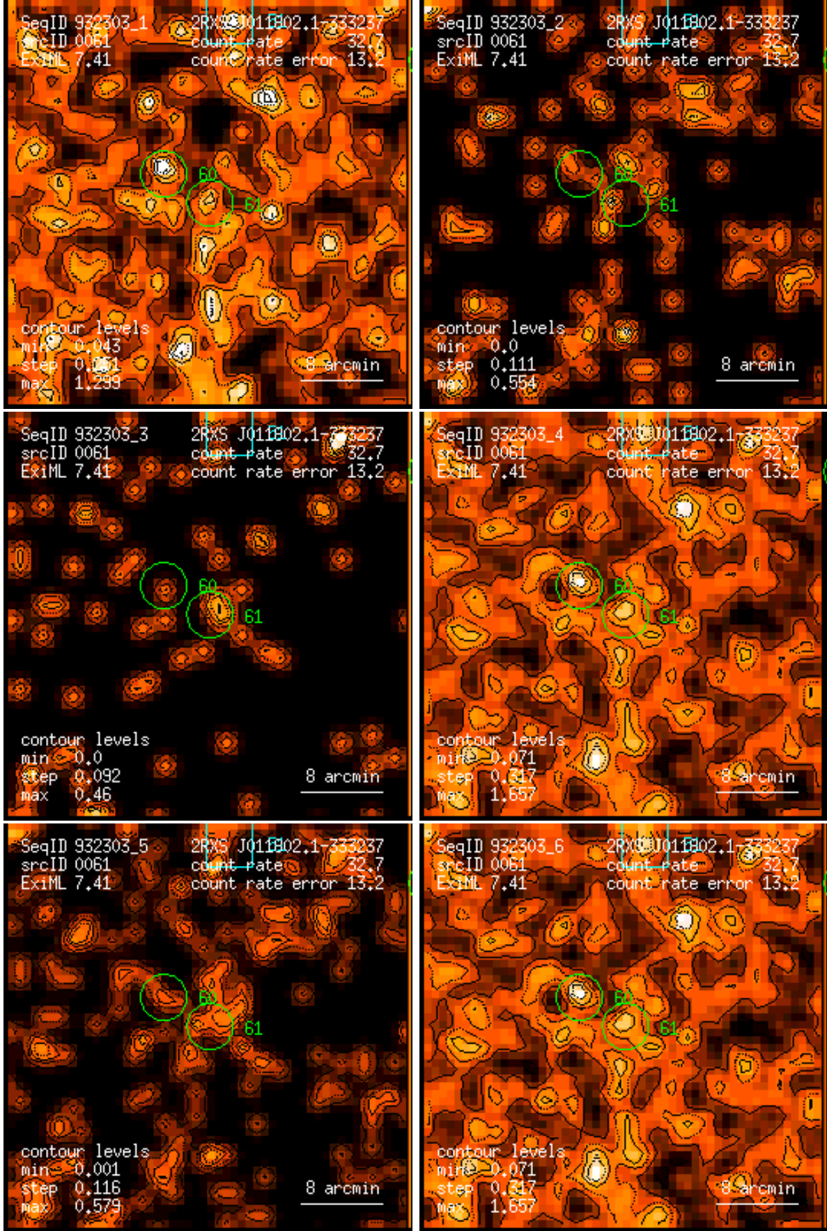
Figure 61: RASS 932303: detection 0061: band rate images, Gaussian filter: (1) PSPC channels 11 – 41, (2) 52 – 90, (3) 91 – 201, (4) 11 – 235, (5) 52 – 201, (6) 11 – 201. Broad band rates in counts/ks. Band rate contour levels in counts/ks/arcmin 2 .
