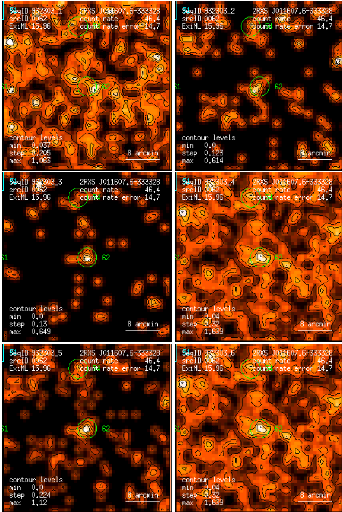
Figure 62: RASS 932303: detection 0062: band rate images, Gaussian filter: (1) PSPC channels 11 – 41, (2) 52 – 90, (3) 91 – 201, (4) 11 – 235, (5) 52 – 201, (6) 11 – 201. Broad band rates in counts/ks. Band rate contour levels in counts/ks/arcmin 2 .
