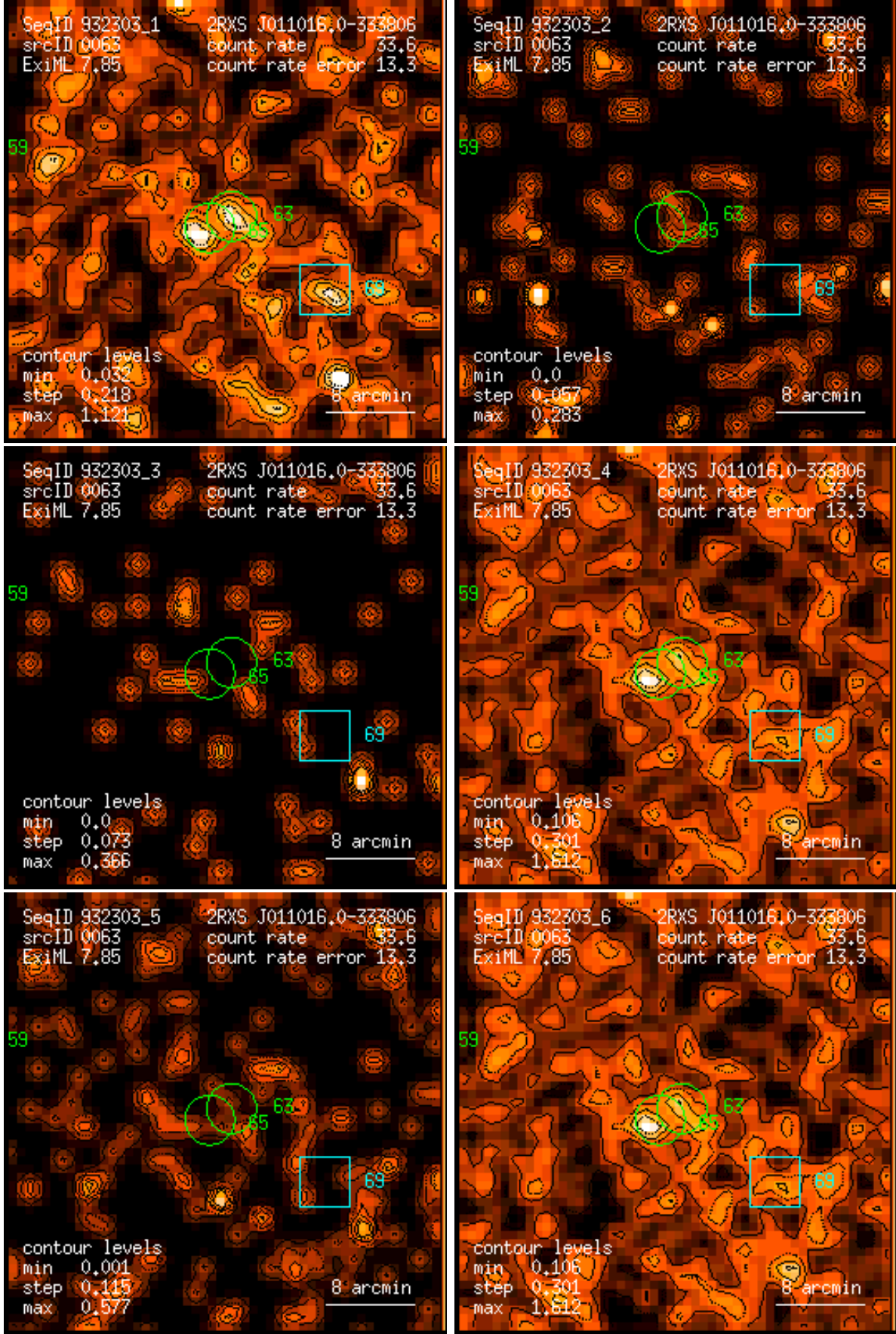
Figure 63: RASS 932303: detection 0063: band rate images, Gaussian filter: (1) PSPC channels 11 – 41, (2) 52 – 90, (3) 91 – 201, (4) 11 – 235, (5) 52 – 201, (6) 11 – 201. Broad band rates in counts/ks. Band rate contour levels in counts/ks/arcmin 2 .
