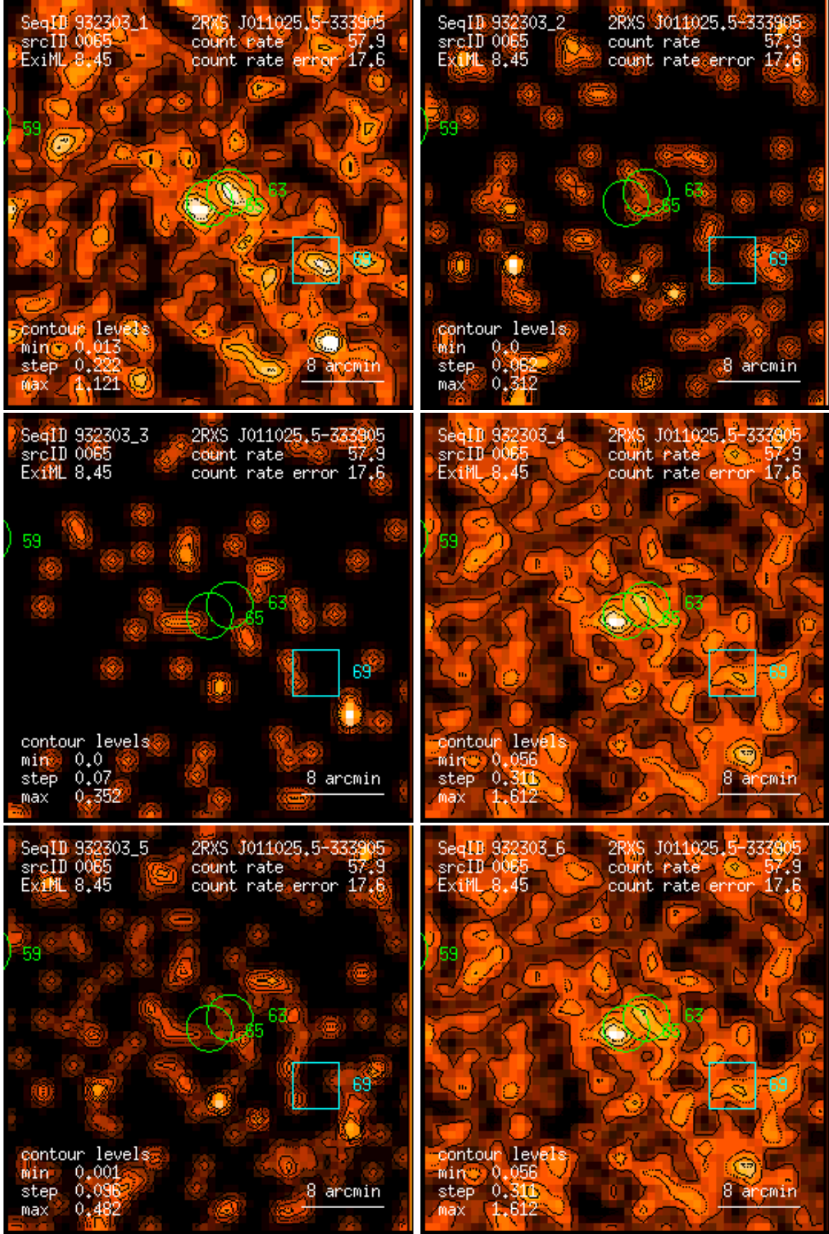
Figure 65: RASS 932303: detection 0065: band rate images, Gaussian filter: (1) PSPC channels 11 – 41, (2) 52 – 90, (3) 91 – 201, (4) 11 – 235, (5) 52 – 201, (6) 11 – 201. Broad band rates in counts/ks. Band rate contour levels in counts/ks/arcmin 2 .
