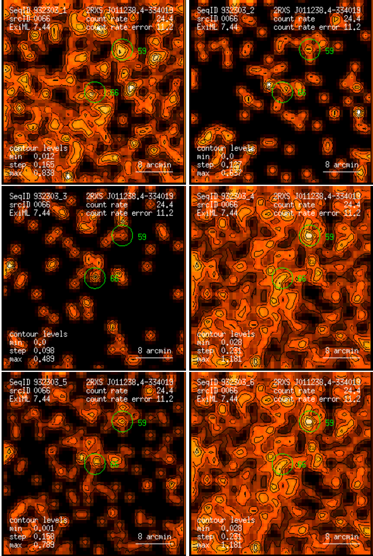
Figure 66: RASS 932303: detection 0066: band rate images, Gaussian filter: (1) PSPC channels 11 – 41, (2) 52 – 90, (3) 91 – 201, (4) 11 – 235, (5) 52 – 201, (6) 11 – 201. Broad band rates in counts/ks. Band rate contour levels in counts/ks/arcmin 2 .
