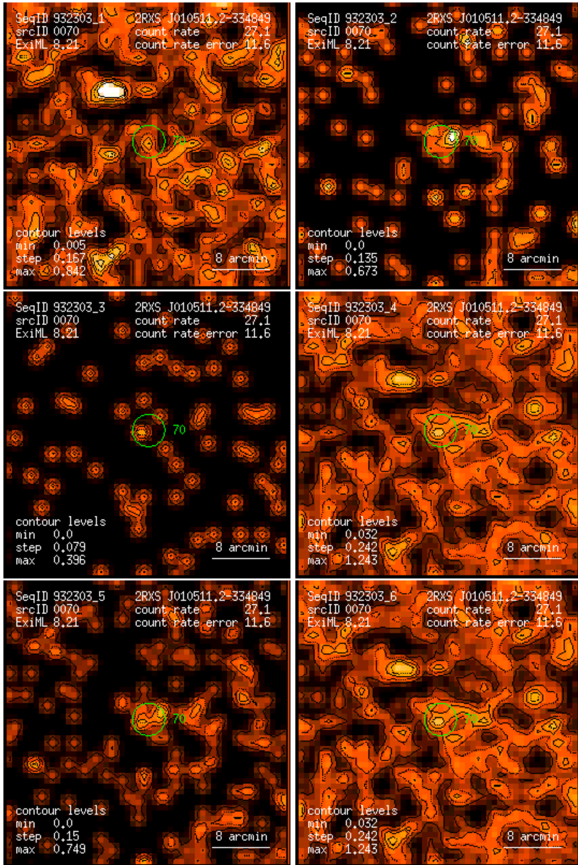
Figure 70: RASS 932303: detection 0070: band rate images, Gaussian filter: (1) PSPC channels 11 – 41, (2) 52 – 90, (3) 91 – 201, (4) 11 – 235, (5) 52 – 201, (6) 11 – 201. Broad band rates in counts/ks. Band rate contour levels in counts/ks/arcmin 2 .
