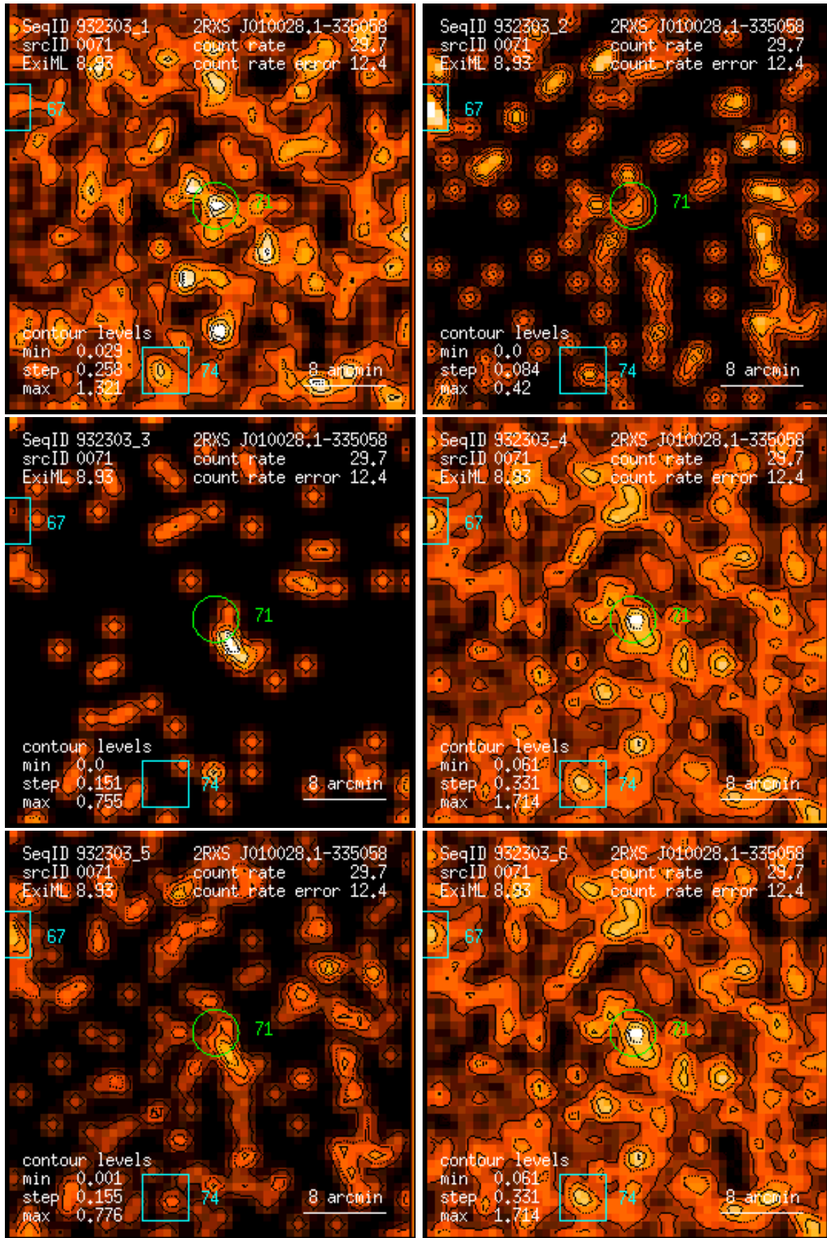
Figure 71: RASS 932303: detection 0071: band rate images, Gaussian filter: (1) PSPC channels 11 – 41, (2) 52 – 90, (3) 91 – 201, (4) 11 – 235, (5) 52 – 201, (6) 11 – 201. Broad band rates in counts/ks. Band rate contour levels in counts/ks/arcmin 2 .
