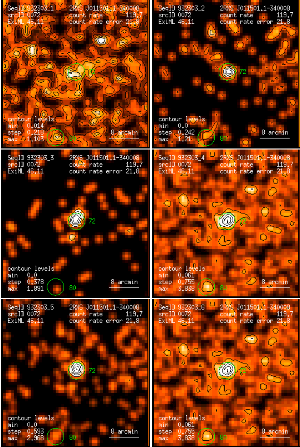
Figure 72: RASS 932303: detection 0072: band rate images, Gaussian filter: (1) PSPC channels 11 – 41, (2) 52 – 90, (3) 91 – 201, (4) 11 – 235, (5) 52 – 201, (6) 11 – 201. Broad band rates in counts/ks. Band rate contour levels in counts/ks/arcmin 2 .
