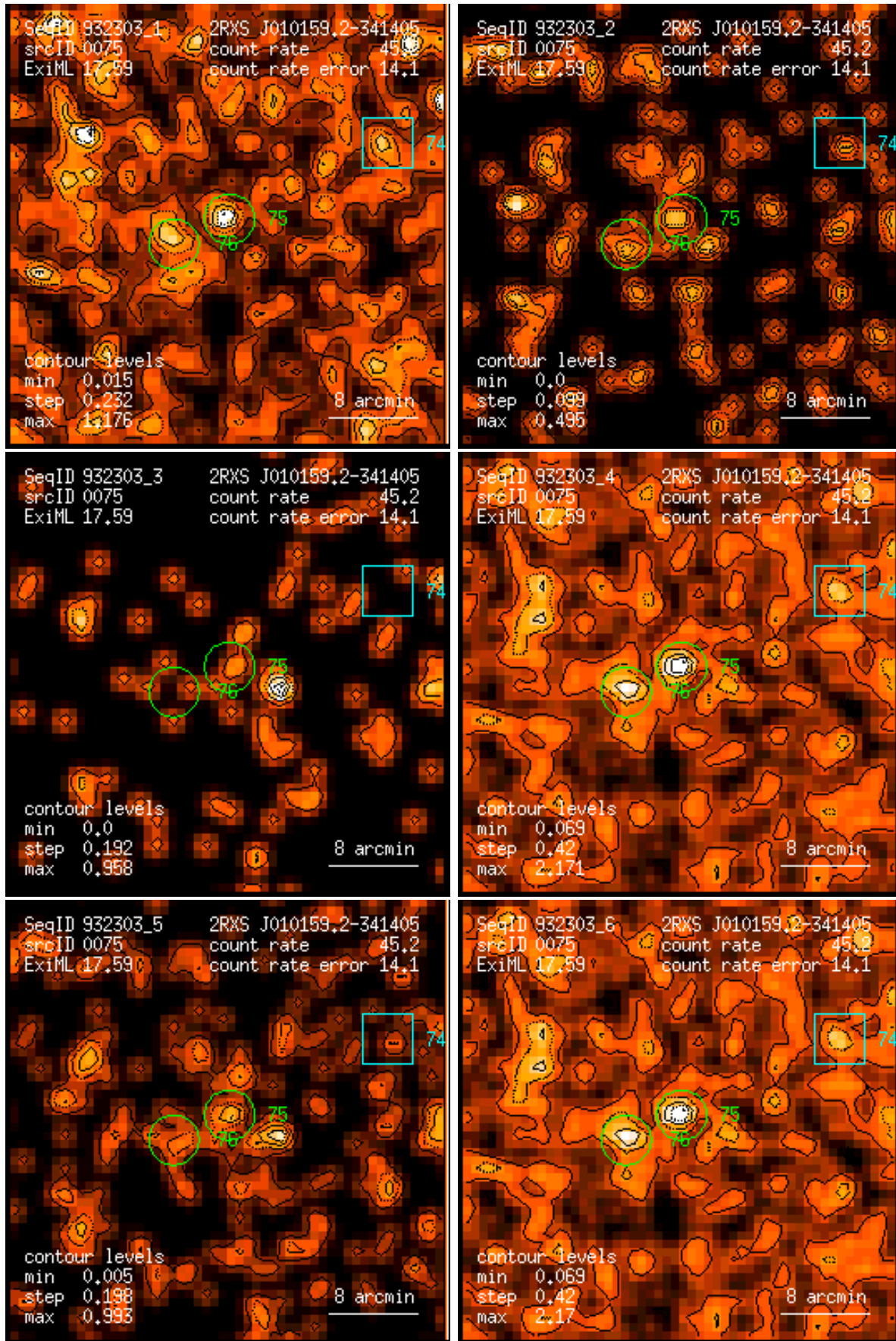
Figure 75: RASS 932303: detection 0075: band rate images, Gaussian filter: (1) PSPC channels 11 – 41, (2) 52 – 90, (3) 91 – 201, (4) 11 – 235, (5) 52 – 201, (6) 11 – 201. Broad band rates in counts/ks. Band rate contour levels in counts/ks/arcmin 2 .
