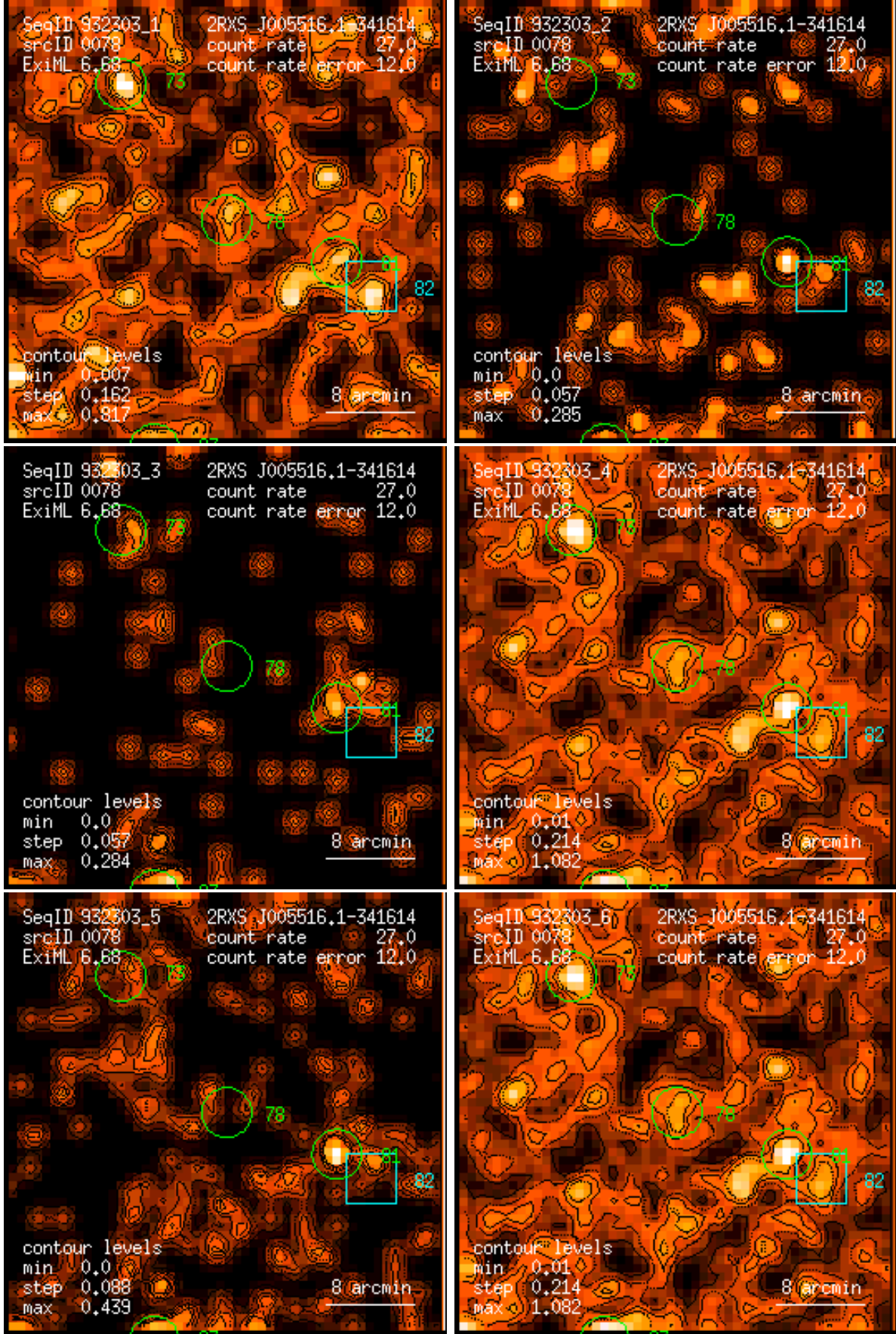
Figure 78: RASS 932303: detection 0078: band rate images, Gaussian filter: (1) PSPC channels 11 – 41, (2) 52 – 90, (3) 91 – 201, (4) 11 – 235, (5) 52 – 201, (6) 11 – 201. Broad band rates in counts/ks. Band rate contour levels in counts/ks/arcmin 2 .
