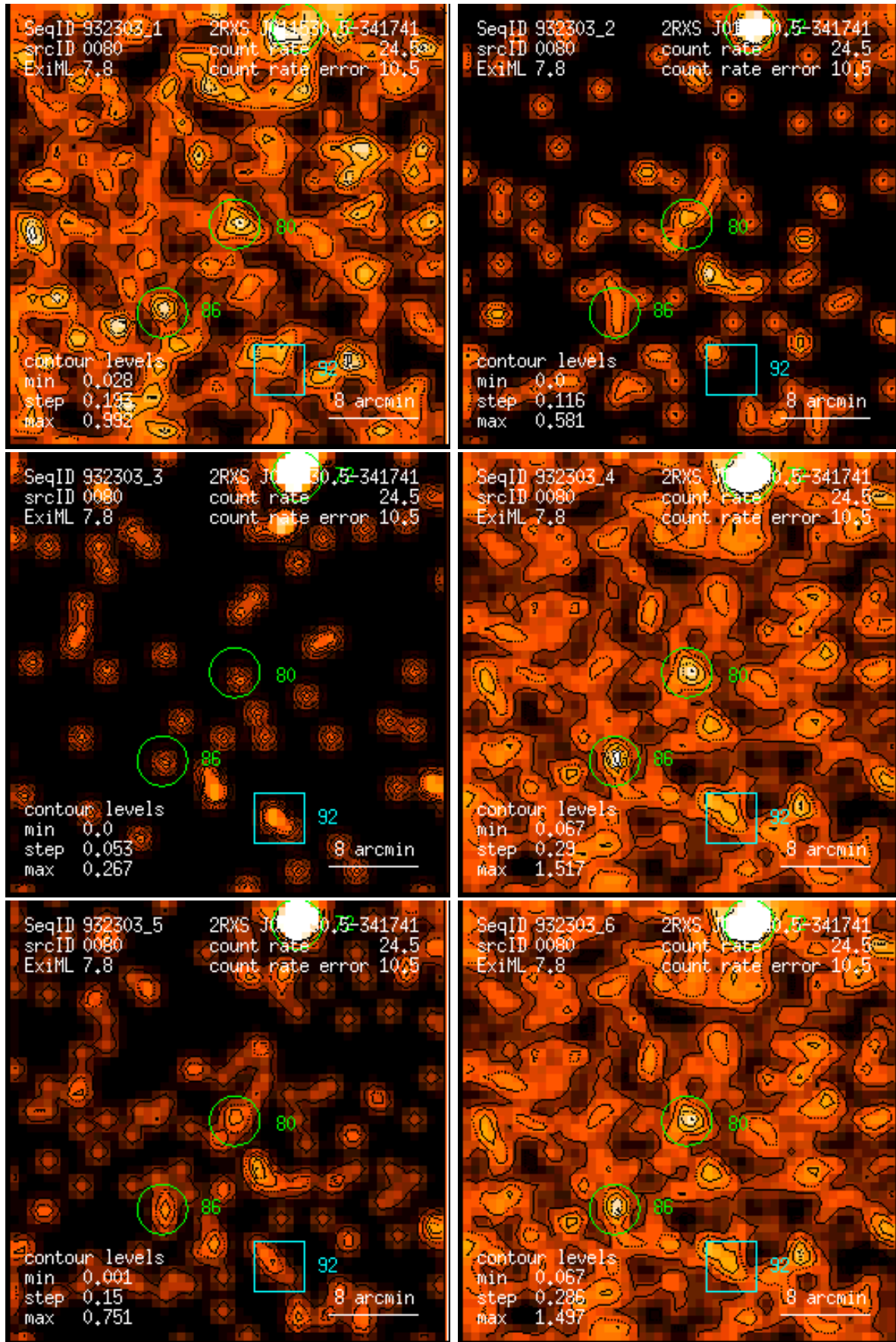
Figure 80: RASS 932303: detection 0080: band rate images, Gaussian filter: (1) PSPC channels 11 – 41, (2) 52 – 90, (3) 91 – 201, (4) 11 – 235, (5) 52 – 201, (6) 11 – 201. Broad band rates in counts/ks. Band rate contour levels in counts/ks/arcmin 2 .
