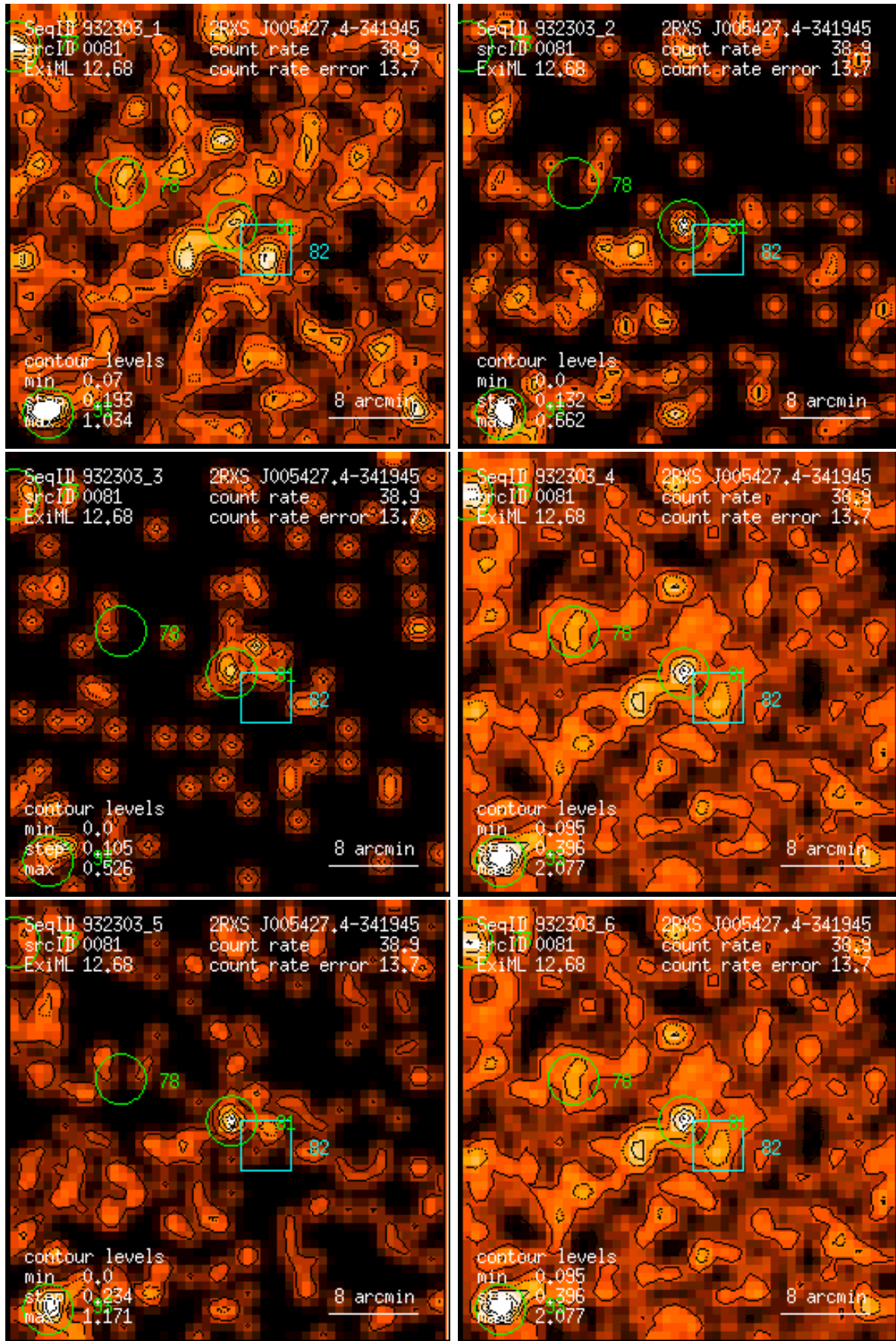
Figure 81: RASS 932303: detection 0081: band rate images, Gaussian filter: (1) PSPC channels 11 – 41, (2) 52 – 90, (3) 91 – 201, (4) 11 – 235, (5) 52 – 201, (6) 11 – 201. Broad band rates in counts/ks. Band rate contour levels in counts/ks/arcmin 2 .
