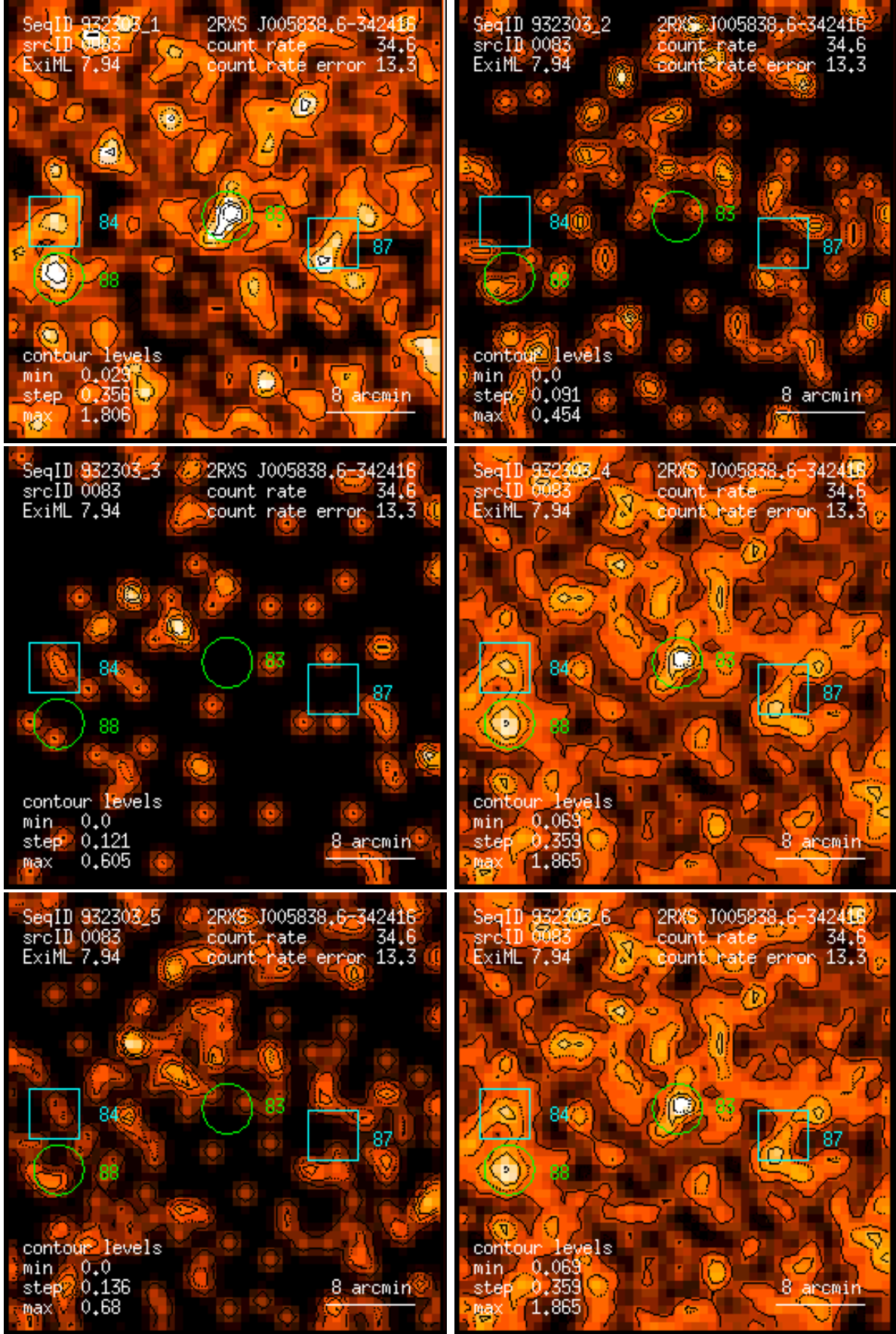
Figure 83: RASS 932303: detection 0083: band rate images, Gaussian filter: (1) PSPC channels 11 – 41, (2) 52 – 90, (3) 91 – 201, (4) 11 – 235, (5) 52 – 201, (6) 11 – 201. Broad band rates in counts/ks. Band rate contour levels in counts/ks/arcmin 2 .
