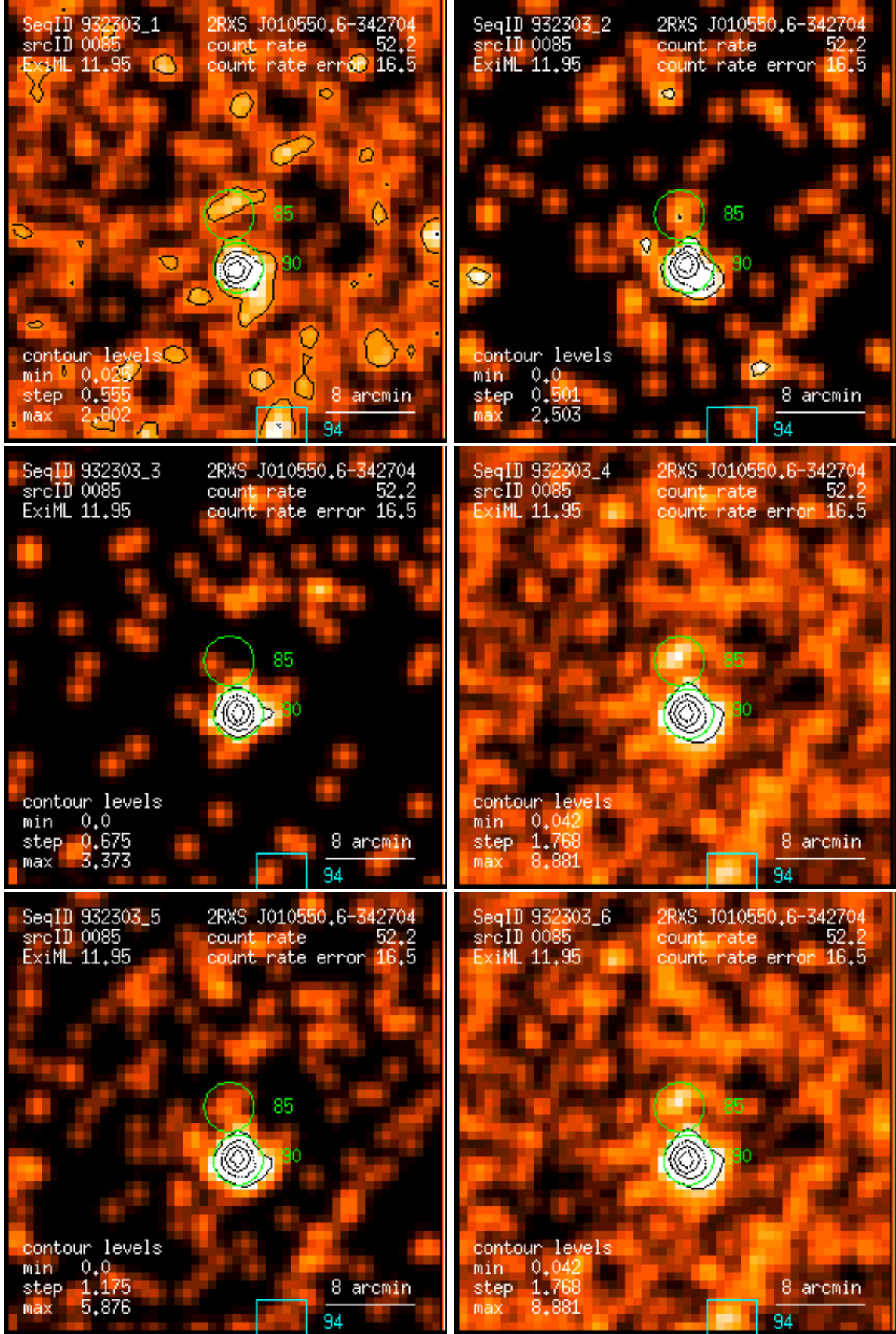
Figure 85: RASS 932303: detection 0085: band rate images, Gaussian filter: (1) PSPC channels 11 – 41, (2) 52 – 90, (3) 91 – 201, (4) 11 – 235, (5) 52 – 201, (6) 11 – 201. Broad band rates in counts/ks. Band rate contour levels in counts/ks/arcmin 2 .
