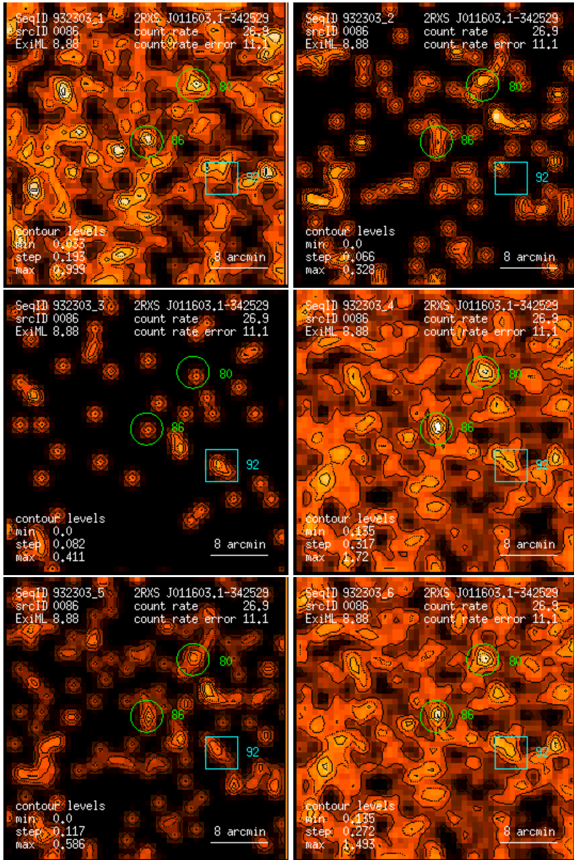
Figure 86: RASS 932303: detection 0086: band rate images, Gaussian filter: (1) PSPC channels 11 – 41, (2) 52 – 90, (3) 91 – 201, (4) 11 – 235, (5) 52 – 201, (6) 11 – 201. Broad band rates in counts/ks. Band rate contour levels in counts/ks/arcmin 2 .
