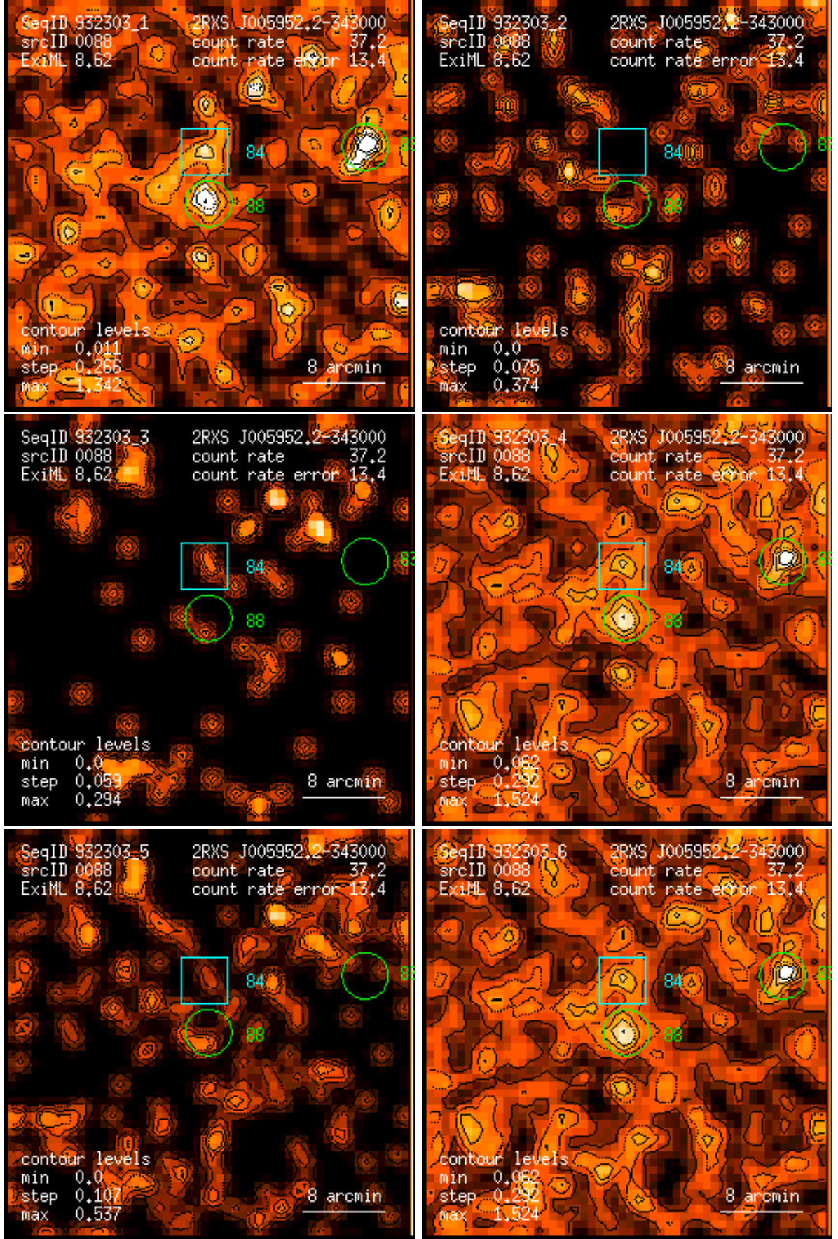
Figure 88: RASS 932303: detection 0088: band rate images, Gaussian filter: (1) PSPC channels 11 – 41, (2) 52 – 90, (3) 91 – 201, (4) 11 – 235, (5) 52 – 201, (6) 11 – 201. Broad band rates in counts/ks. Band rate contour levels in counts/ks/arcmin 2 .
